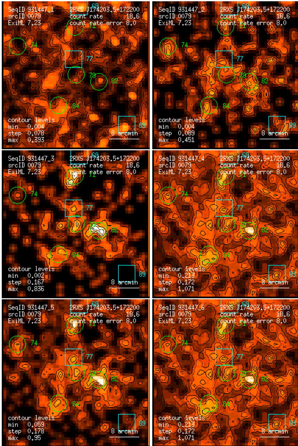
Figure 79: RASS 931447: detection 0079: band rate images, Gaussian filter: (1) PSPC channels 11 – 41, (2) 52 – 90, (3) 91 – 201, (4) 11 – 235, (5) 52 – 201, (6) 11 – 201. Broad band rates in counts/ks. Band rate contour levels in counts/ks/arcmin 2 .
