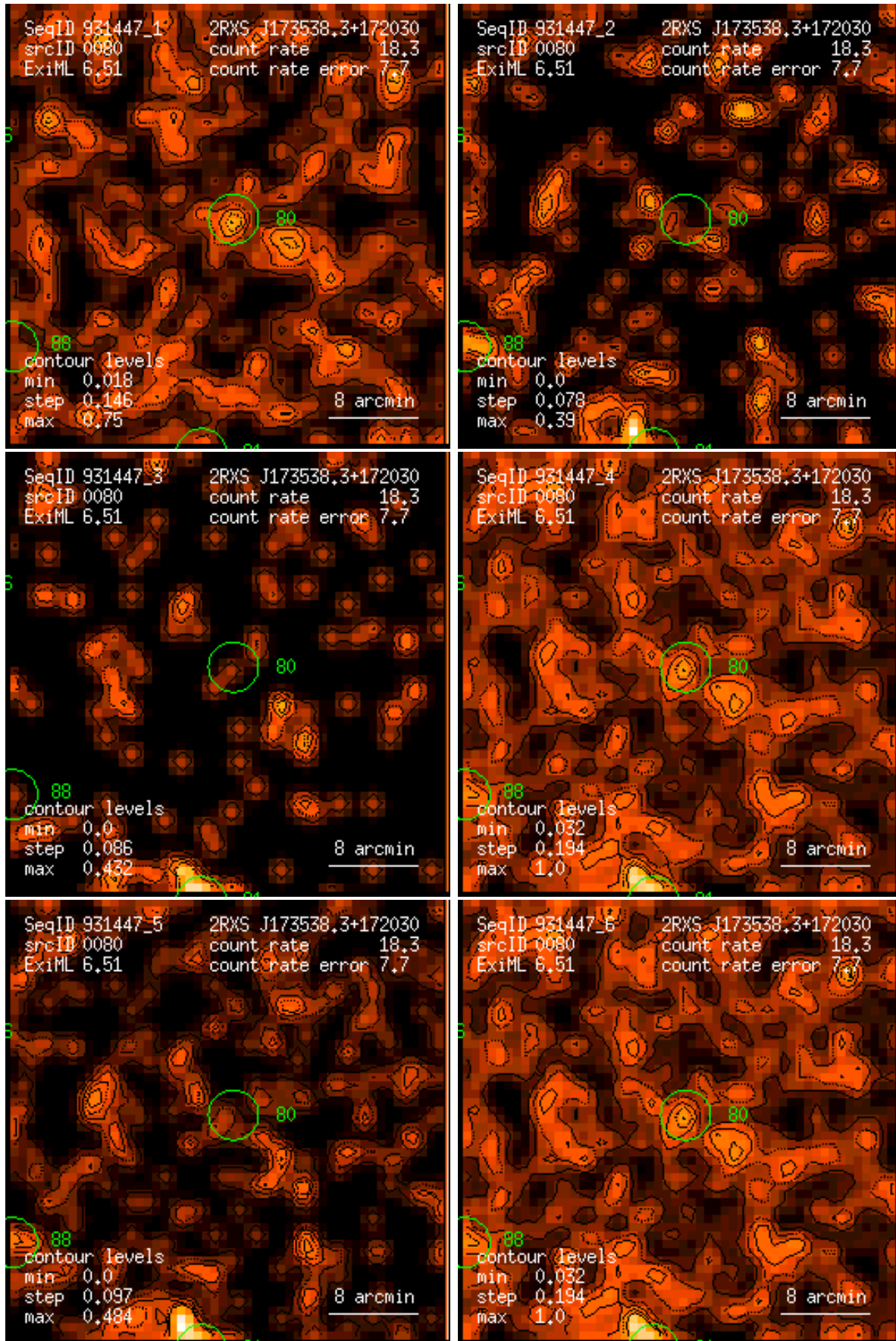
Figure 80: RASS 931447: detection 0080: band rate images, Gaussian filter: (1) PSPC channels 11 – 41, (2) 52 – 90, (3) 91 – 201, (4) 11 – 235, (5) 52 – 201, (6) 11 – 201. Broad band rates in counts/ks. Band rate contour levels in counts/ks/arcmin 2 .
