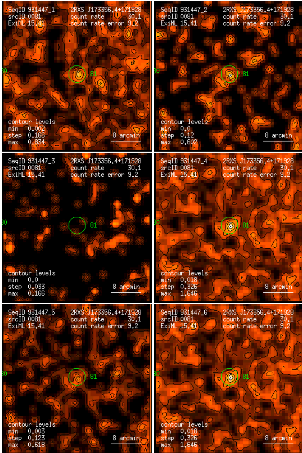
Figure 81: RASS 931447: detection 0081: band rate images, Gaussian filter: (1) PSPC channels 11 – 41, (2) 52 – 90, (3) 91 – 201, (4) 11 – 235, (5) 52 – 201, (6) 11 – 201. Broad band rates in counts/ks. Band rate contour levels in counts/ks/arcmin 2 .
