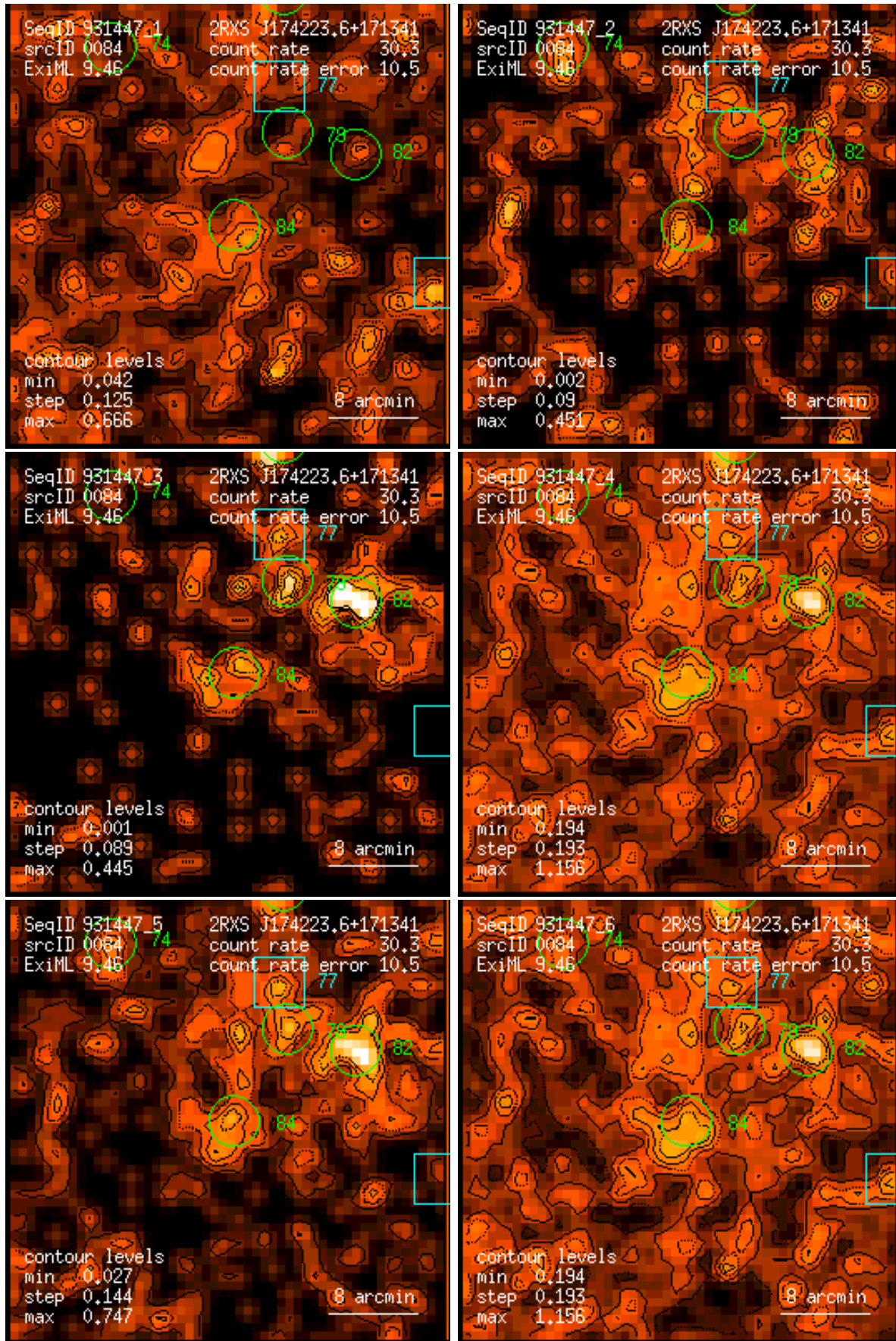
Figure 84: RASS 931447: detection 0084: band rate images, Gaussian filter: (1) PSPC channels 11 – 41, (2) 52 – 90, (3) 91 – 201, (4) 11 – 235, (5) 52 – 201, (6) 11 – 201. Broad band rates in counts/ks. Band rate contour levels in counts/ks/arcmin 2 .
