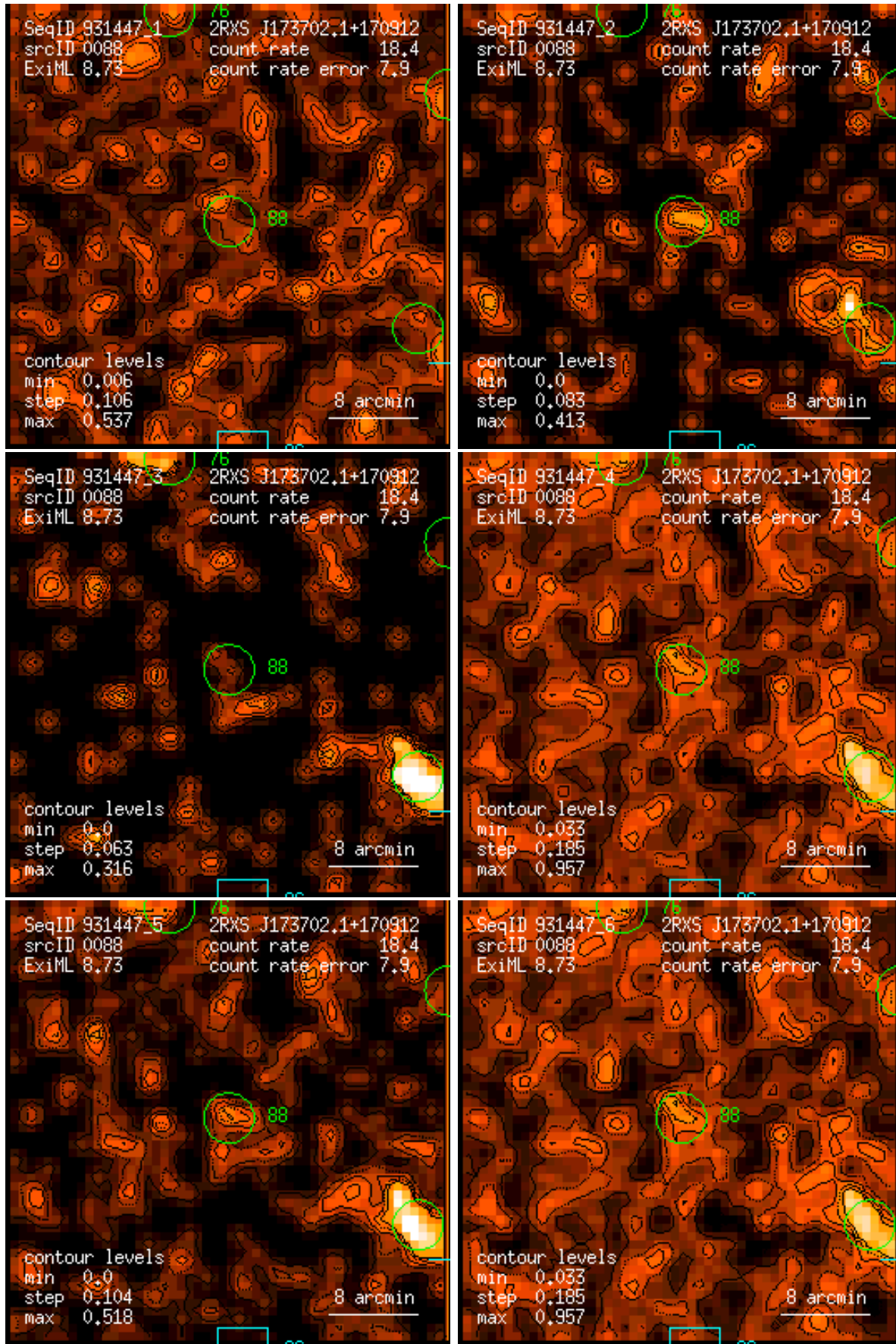
Figure 88: RASS 931447: detection 0088: band rate images, Gaussian filter: (1) PSPC channels 11 – 41, (2) 52 – 90, (3) 91 – 201, (4) 11 – 235, (5) 52 – 201, (6) 11 – 201. Broad band rates in counts/ks. Band rate contour levels in counts/ks/arcmin 2 .
