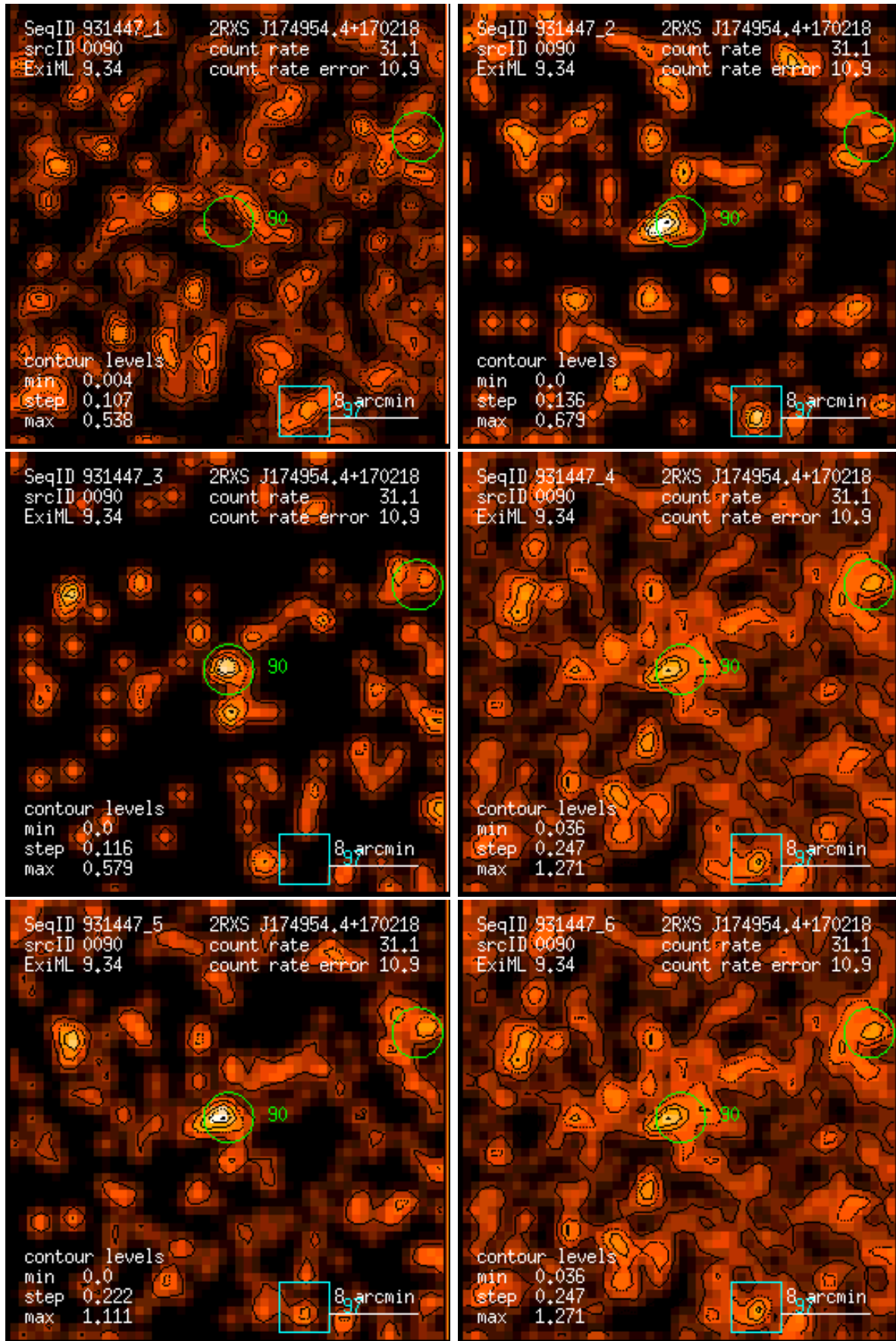
Figure 90: RASS 931447: detection 0090: band rate images, Gaussian filter: (1) PSPC channels 11 – 41, (2) 52 – 90, (3) 91 – 201, (4) 11 – 235, (5) 52 – 201, (6) 11 – 201. Broad band rates in counts/ks. Band rate contour levels in counts/ks/arcmin 2 .
