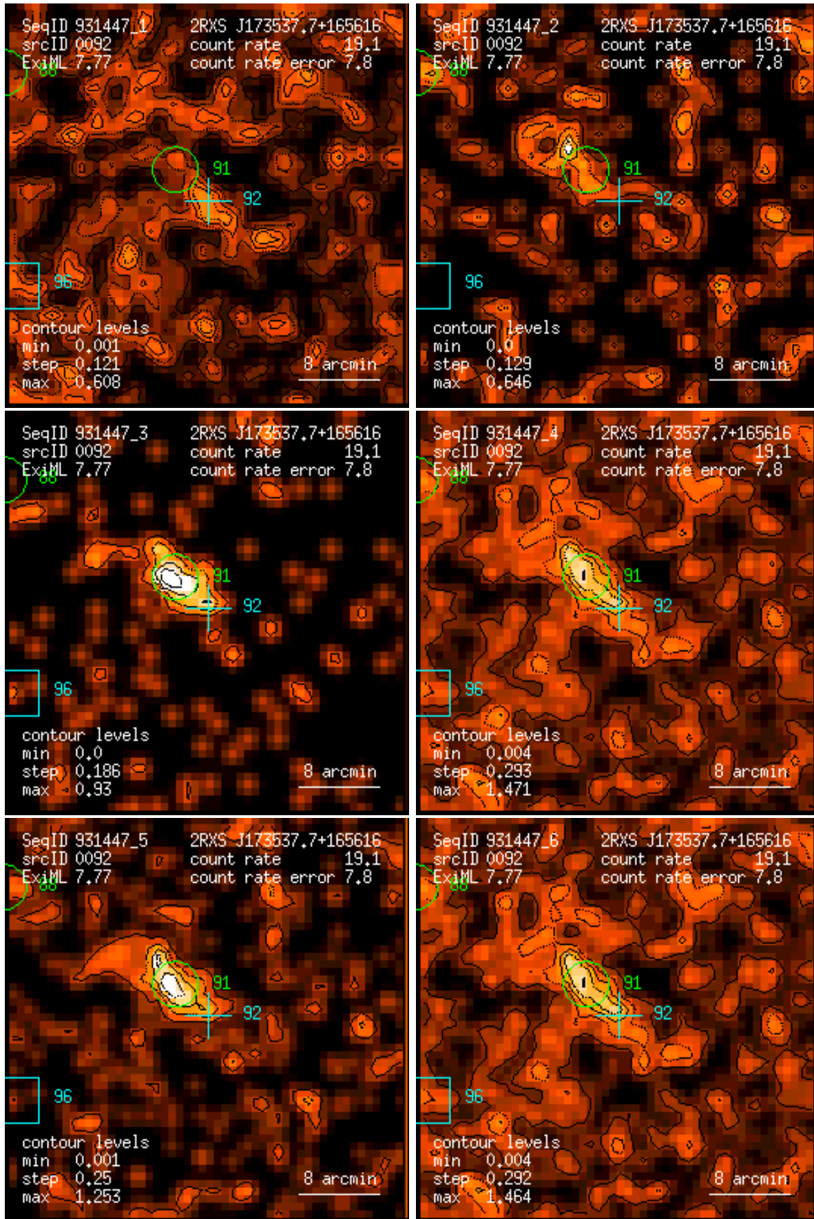
Figure 92: RASS 931447: detection 0092: band rate images, Gaussian filter: (1) PSPC channels 11 – 41, (2) 52 – 90, (3) 91 – 201, (4) 11 – 235, (5) 52 – 201, (6) 11 – 201. Broad band rates in counts/ks. Band rate contour levels in counts/ks/arcmin 2 .
