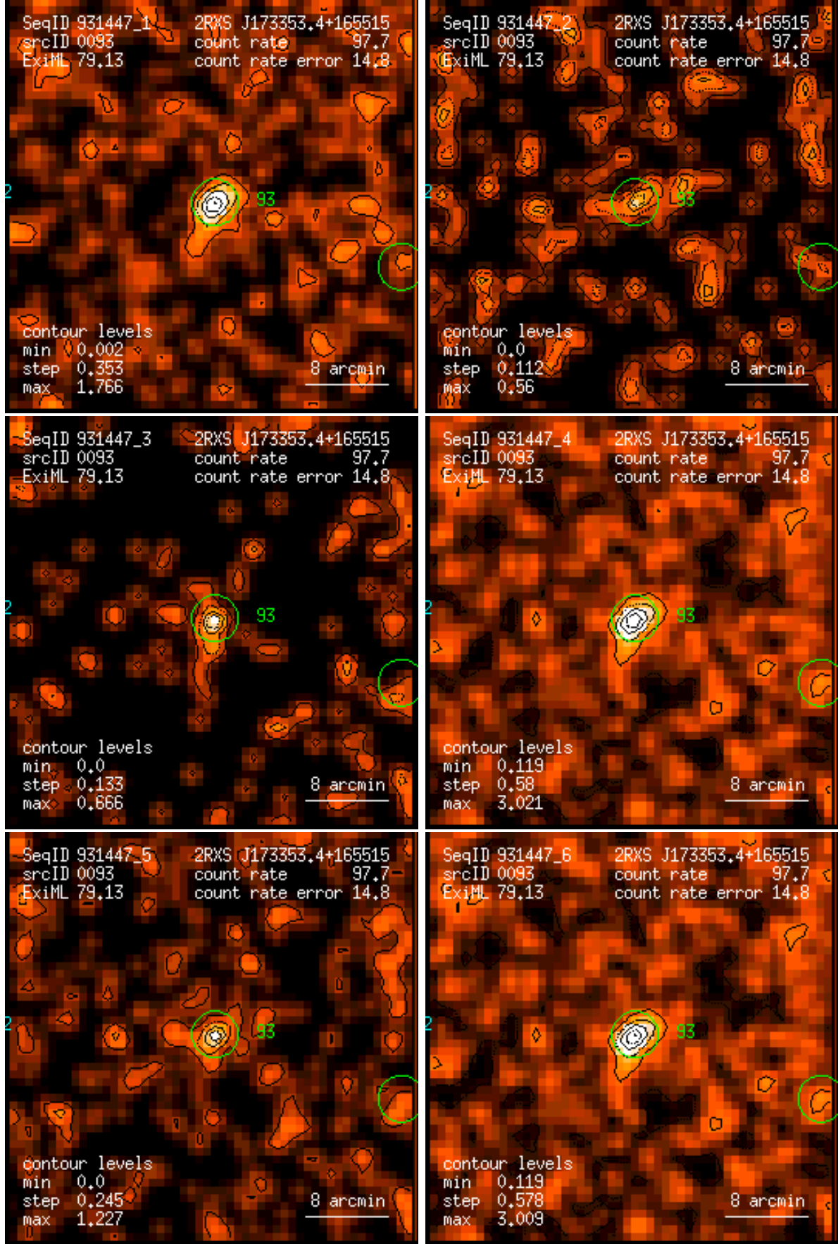
Figure 93: RASS 931447: detection 0093: band rate images, Gaussian filter: (1) PSPC channels 11 – 41, (2) 52 – 90, (3) 91 – 201, (4) 11 – 235, (5) 52 – 201, (6) 11 – 201. Broad band rates in counts/ks. Band rate contour levels in counts/ks/arcmin 2 .
