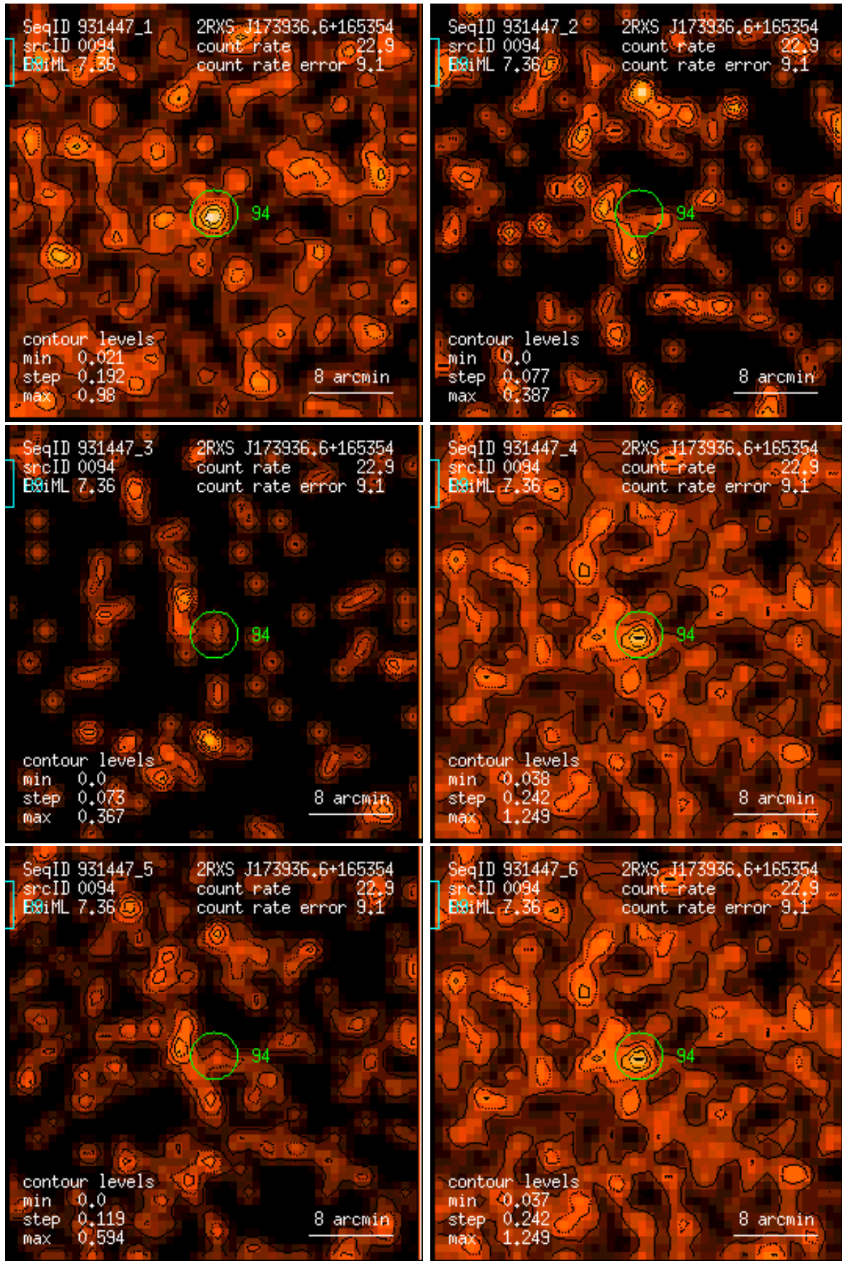
Figure 94: RASS 931447: detection 0094: band rate images, Gaussian filter: (1) PSPC channels 11 – 41, (2) 52 – 90, (3) 91 – 201, (4) 11 – 235, (5) 52 – 201, (6) 11 – 201. Broad band rates in counts/ks. Band rate contour levels in counts/ks/arcmin 2 .
