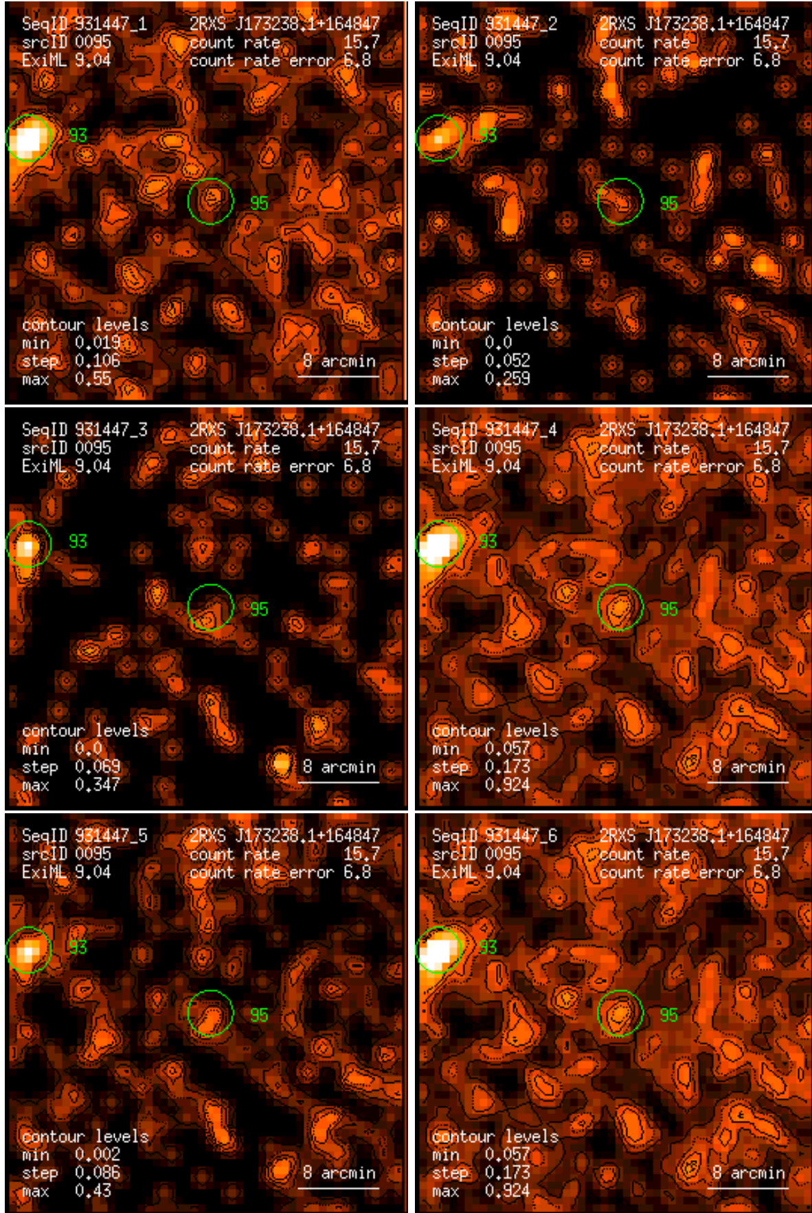
Figure 95: RASS 931447: detection 0095: band rate images, Gaussian filter: (1) PSPC channels 11 – 41, (2) 52 – 90, (3) 91 – 201, (4) 11 – 235, (5) 52 – 201, (6) 11 – 201. Broad band rates in counts/ks. Band rate contour levels in counts/ks/arcmin 2 .
