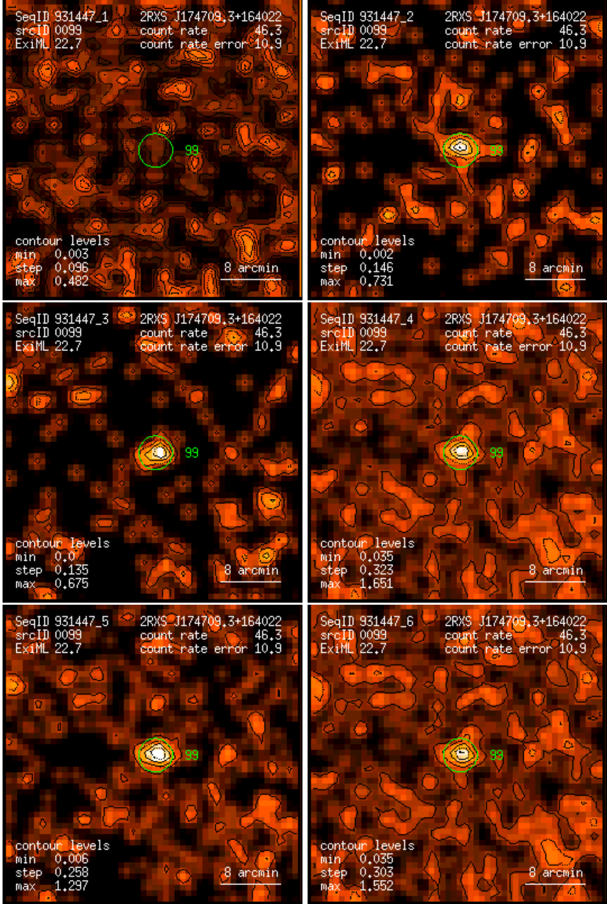
Figure 99: RASS 931447: detection 0099: band rate images, Gaussian filter: (1) PSPC channels 11 – 41, (2) 52 – 90, (3) 91 – 201, (4) 11 – 235, (5) 52 – 201, (6) 11 – 201. Broad band rates in counts/ks. Band rate contour levels in counts/ks/arcmin 2 .
