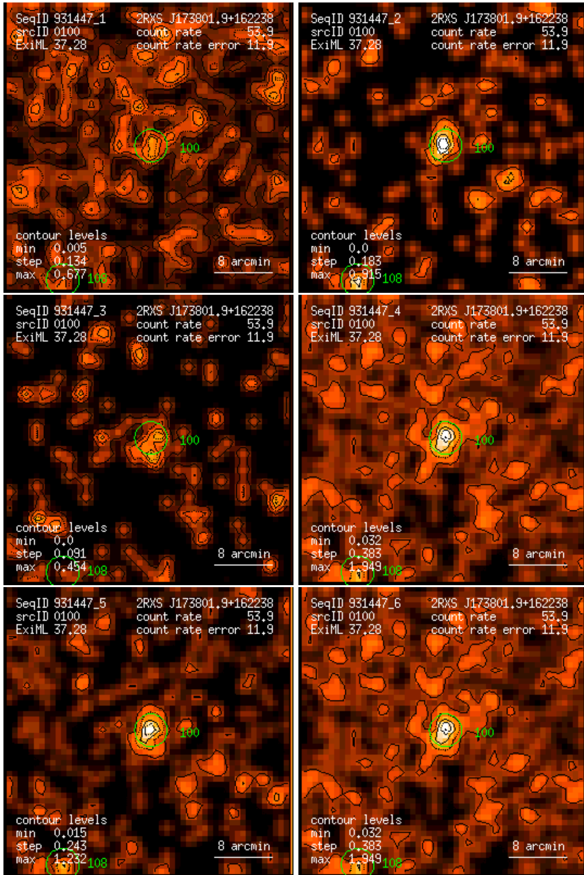
Figure 100: RASS 931447: detection 0100: band rate images, Gaussian filter: (1) PSPC channels 11 – 41, (2) 52 – 90, (3) 91 – 201, (4) 11 – 235, (5) 52 – 201, (6) 11 – 201. Broad band rates in counts/ks. Band rate contour levels in counts/ks/arcmin 2 .
