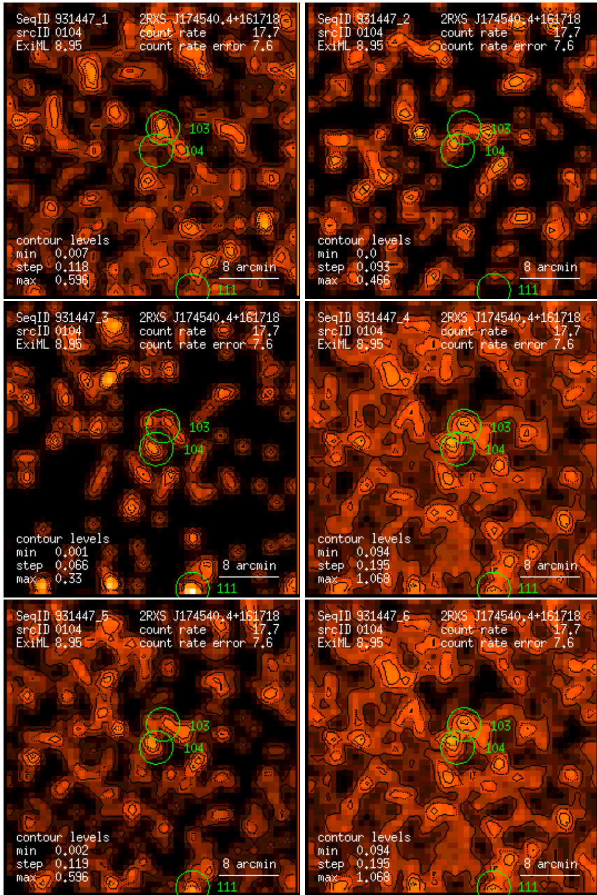
Figure 104: RASS 931447: detection 0104: band rate images, Gaussian filter: (1) PSPC channels 11 – 41, (2) 52 – 90, (3) 91 – 201, (4) 11 – 235, (5) 52 – 201, (6) 11 – 201. Broad band rates in counts/ks. Band rate contour levels in counts/ks/arcmin 2 .
