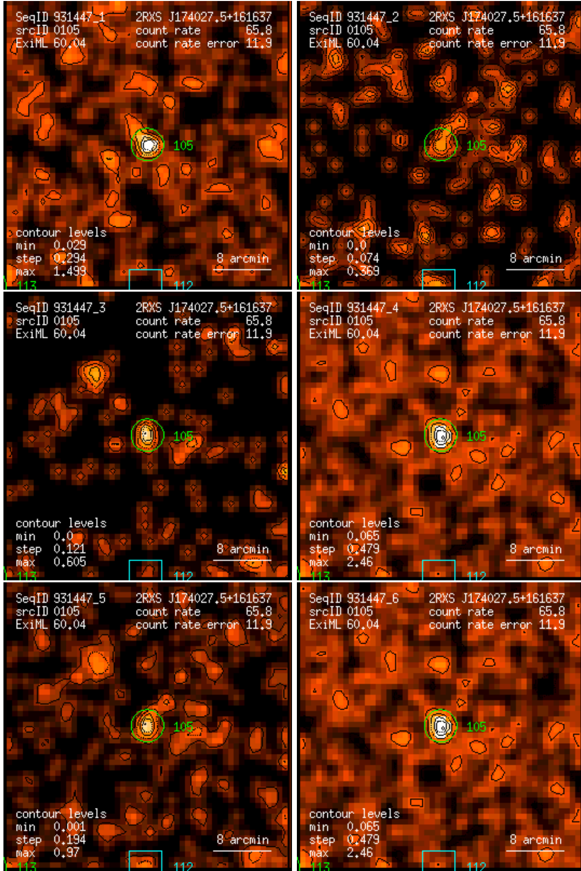
Figure 105: RASS 931447: detection 0105: band rate images, Gaussian filter: (1) PSPC channels 11 – 41, (2) 52 – 90, (3) 91 – 201, (4) 11 – 235, (5) 52 – 201, (6) 11 – 201. Broad band rates in counts/ks. Band rate contour levels in counts/ks/arcmin 2 .
