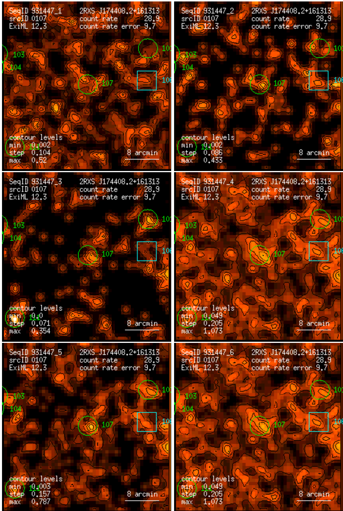
Figure 107: RASS 931447: detection 0107: band rate images, Gaussian filter: (1) PSPC channels 11 – 41, (2) 52 – 90, (3) 91 – 201, (4) 11 – 235, (5) 52 – 201, (6) 11 – 201. Broad band rates in counts/ks. Band rate contour levels in counts/ks/arcmin 2 .
