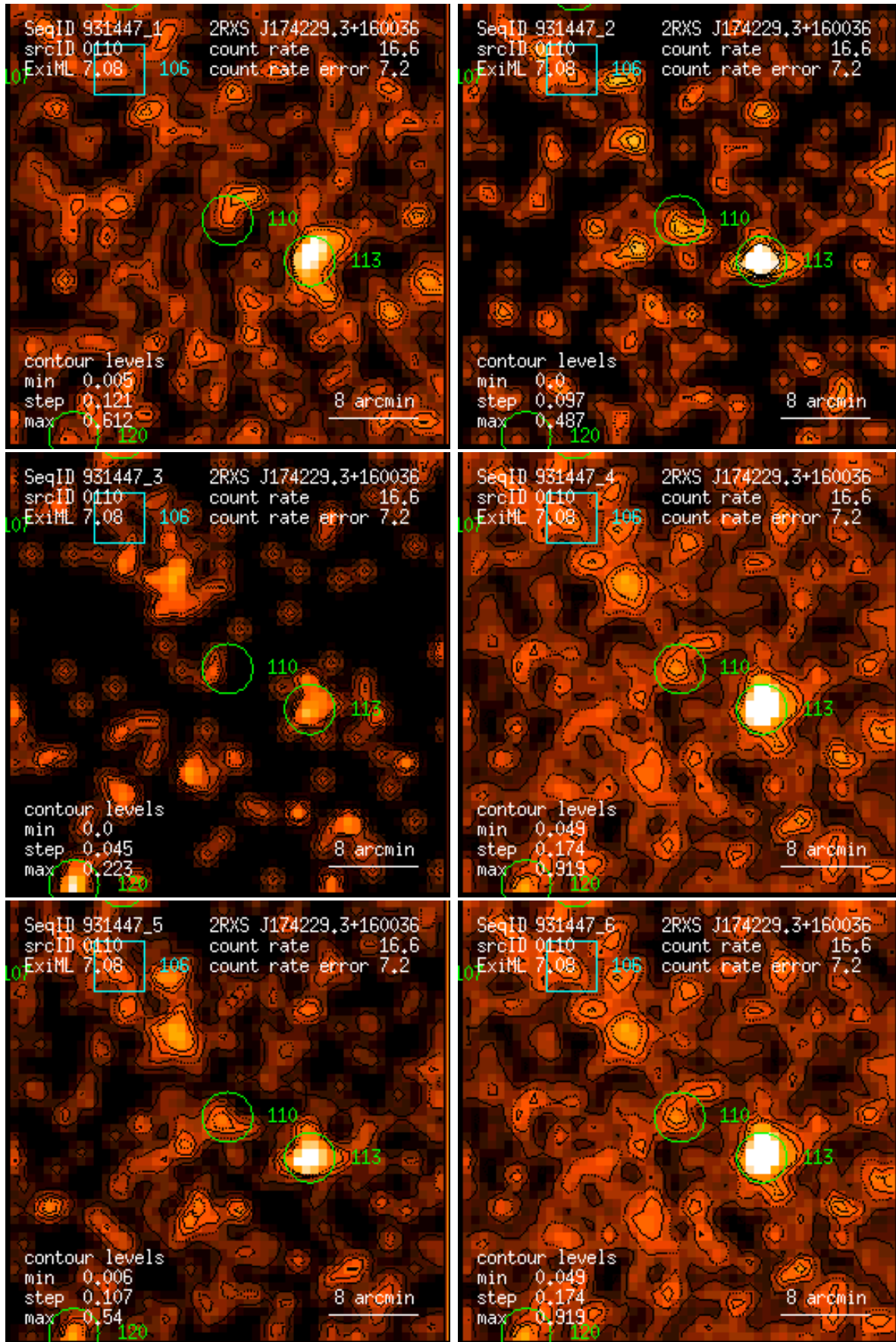
Figure 110: RASS 931447: detection 0110: band rate images, Gaussian filter: (1) PSPC channels 11 – 41, (2) 52 – 90, (3) 91 – 201, (4) 11 – 235, (5) 52 – 201, (6) 11 – 201. Broad band rates in counts/ks. Band rate contour levels in counts/ks/arcmin 2 .
