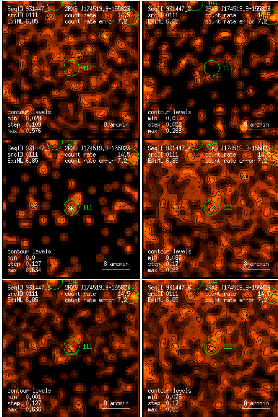
Figure 111: RASS 931447: detection 0111: band rate images, Gaussian filter: (1) PSPC channels 11 – 41, (2) 52 – 90, (3) 91 – 201, (4) 11 – 235, (5) 52 – 201, (6) 11 – 201. Broad band rates in counts/ks. Band rate contour levels in counts/ks/arcmin 2 .
