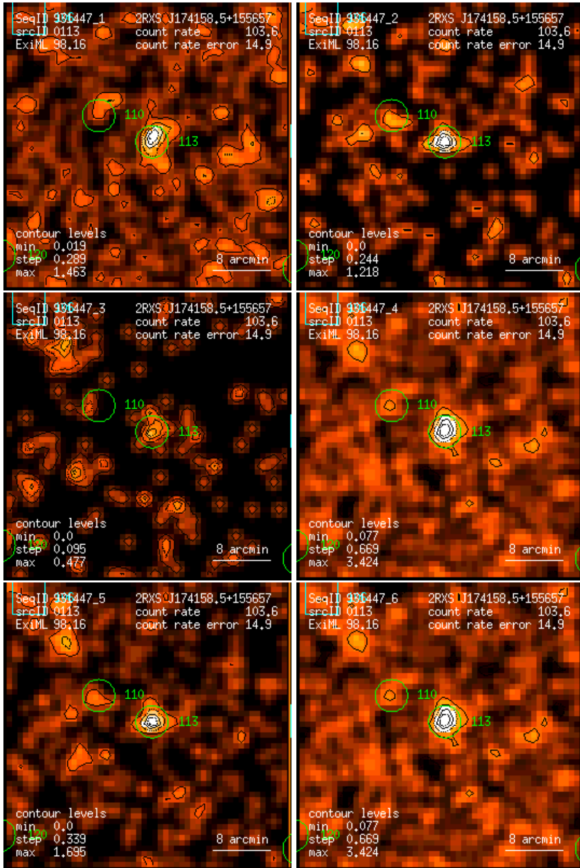
Figure 113: RASS 931447: detection 0113: band rate images, Gaussian filter: (1) PSPC channels 11 – 41, (2) 52 – 90, (3) 91 – 201, (4) 11 – 235, (5) 52 – 201, (6) 11 – 201. Broad band rates in counts/ks. Band rate contour levels in counts/ks/arcmin 2 .
