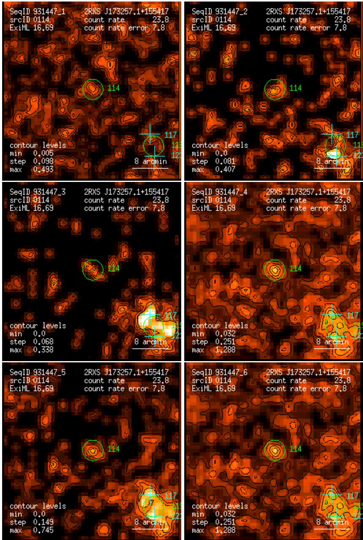
Figure 114: RASS 931447: detection 0114: band rate images, Gaussian filter: (1) PSPC channels 11 – 41, (2) 52 – 90, (3) 91 – 201, (4) 11 – 235, (5) 52 – 201, (6) 11 – 201. Broad band rates in counts/ks. Band rate contour levels in counts/ks/arcmin 2 .
