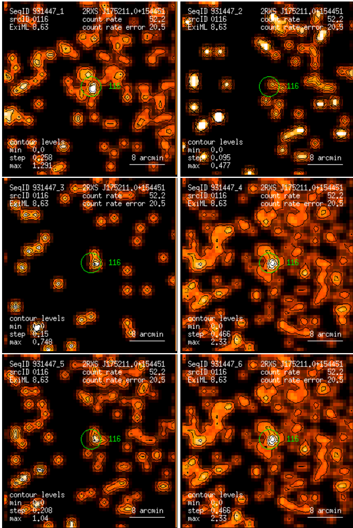
Figure 116: RASS 931447: detection 0116: band rate images, Gaussian filter: (1) PSPC channels 11 – 41, (2) 52 – 90, (3) 91 – 201, (4) 11 – 235, (5) 52 – 201, (6) 11 – 201. Broad band rates in counts/ks. Band rate contour levels in counts/ks/arcmin 2 .
