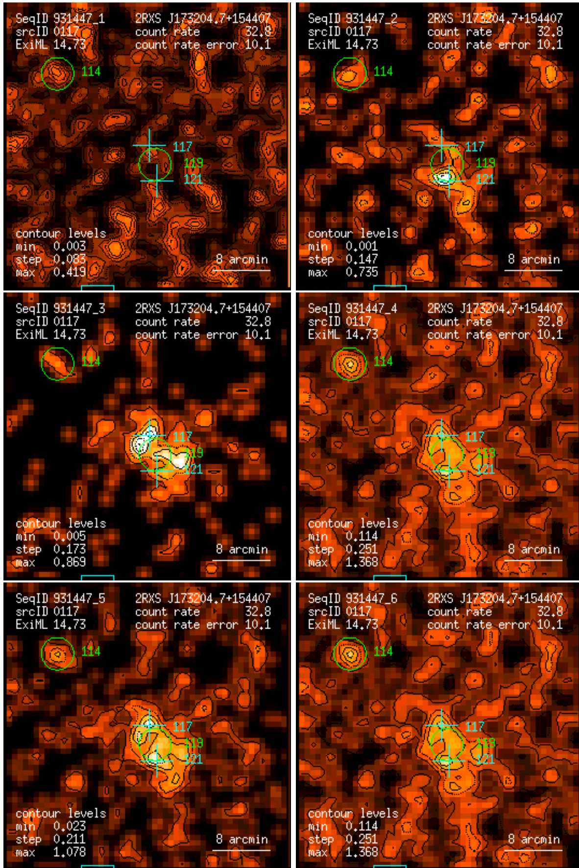
Figure 117: RASS 931447: detection 0117: band rate images, Gaussian filter: (1) PSPC channels 11 – 41, (2) 52 – 90, (3) 91 – 201, (4) 11 – 235, (5) 52 – 201, (6) 11 – 201. Broad band rates in counts/ks. Band rate contour levels in counts/ks/arcmin 2 .
