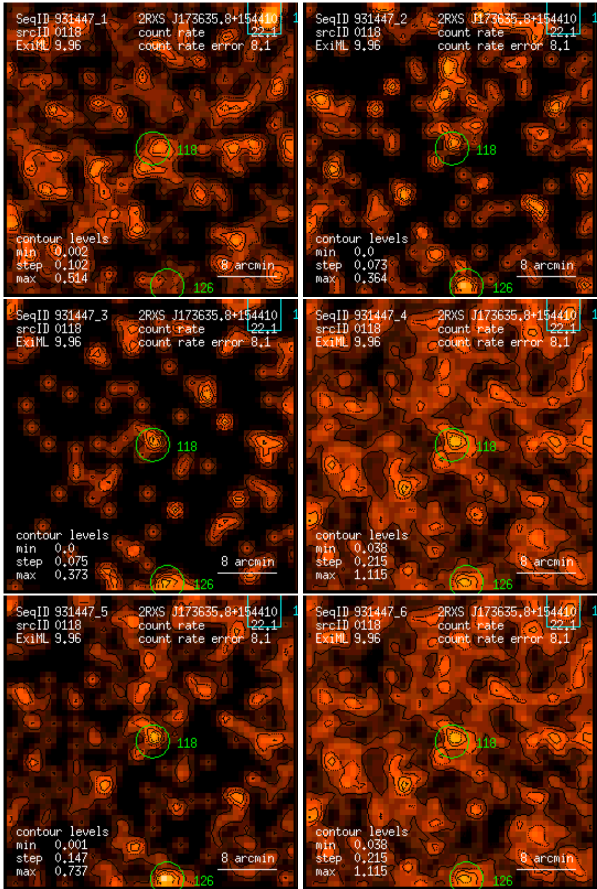
Figure 118: RASS 931447: detection 0118: band rate images, Gaussian filter: (1) PSPC channels 11 – 41, (2) 52 – 90, (3) 91 – 201, (4) 11 – 235, (5) 52 – 201, (6) 11 – 201. Broad band rates in counts/ks. Band rate contour levels in counts/ks/arcmin 2 .
