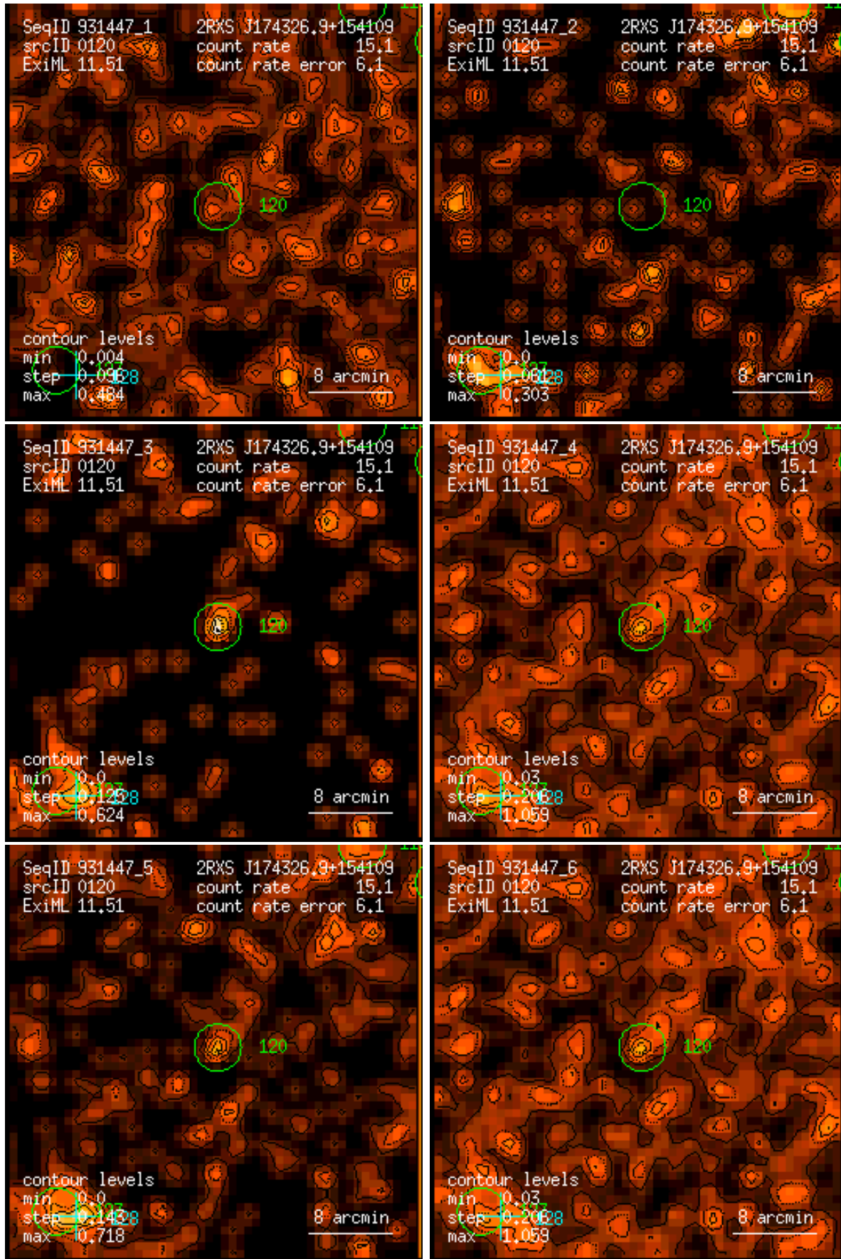
Figure 120: RASS 931447: detection 0120: band rate images, Gaussian filter: (1) PSPC channels 11 – 41, (2) 52 – 90, (3) 91 – 201, (4) 11 – 235, (5) 52 – 201, (6) 11 – 201. Broad band rates in counts/ks. Band rate contour levels in counts/ks/arcmin 2 .
