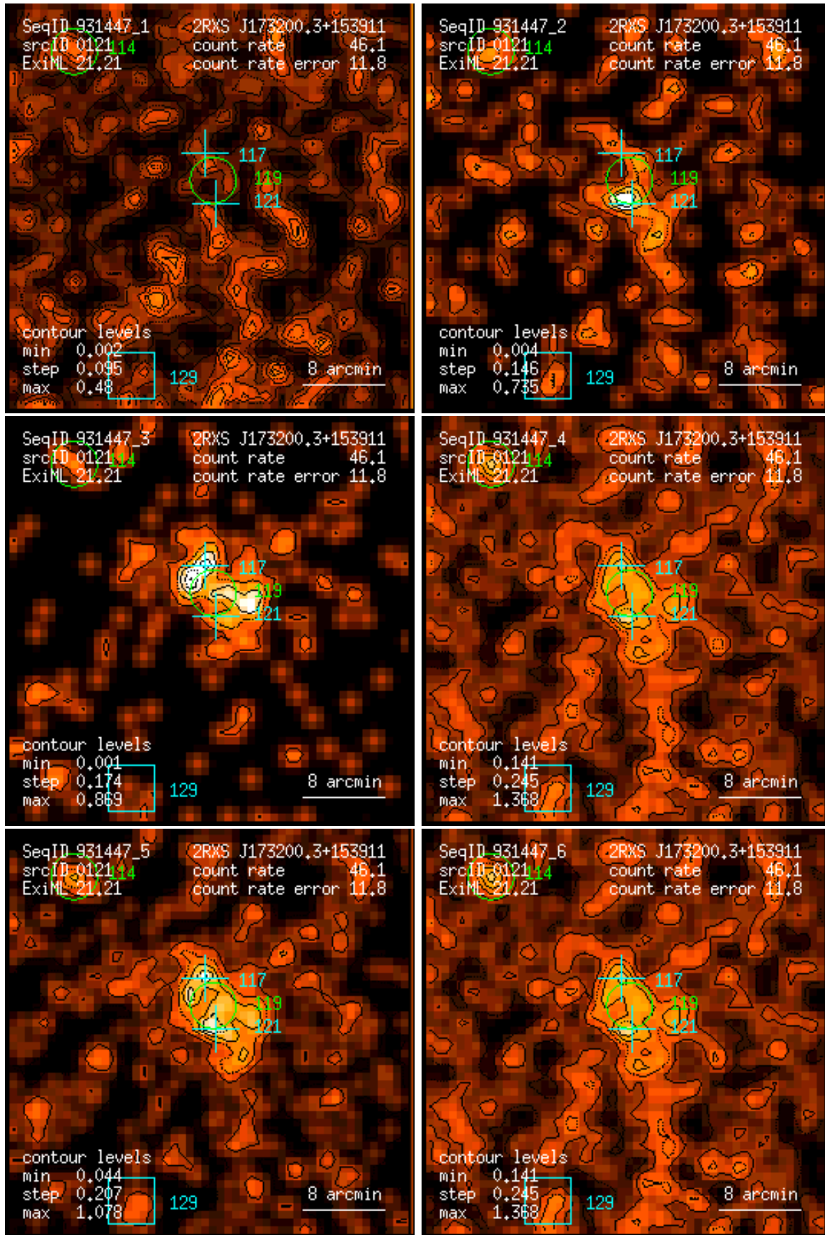
Figure 121: RASS 931447: detection 0121: band rate images, Gaussian filter: (1) PSPC channels 11 – 41, (2) 52 – 90, (3) 91 – 201, (4) 11 – 235, (5) 52 – 201, (6) 11 – 201. Broad band rates in counts/ks. Band rate contour levels in counts/ks/arcmin 2 .
