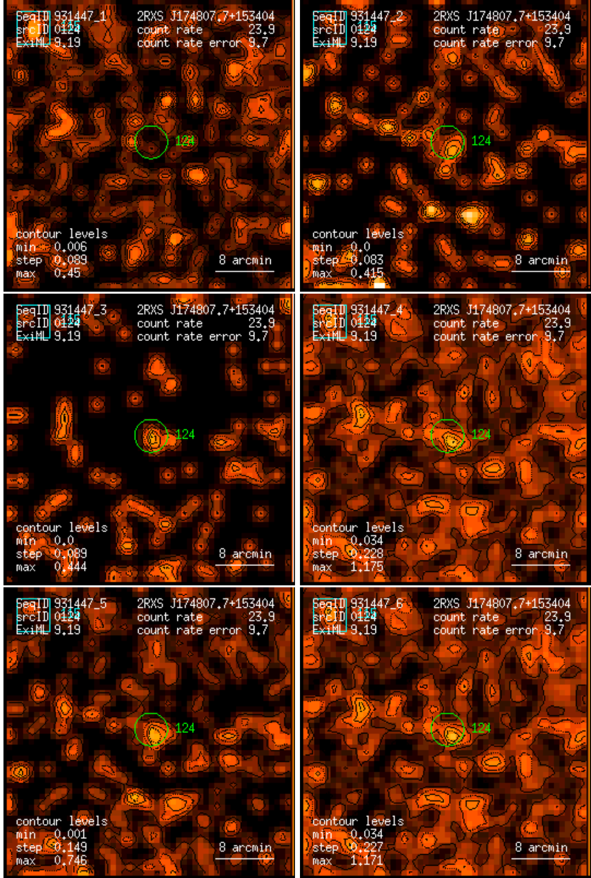
Figure 124: RASS 931447: detection 0124: band rate images, Gaussian filter: (1) PSPC channels 11 – 41, (2) 52 – 90, (3) 91 – 201, (4) 11 – 235, (5) 52 – 201, (6) 11 – 201. Broad band rates in counts/ks. Band rate contour levels in counts/ks/arcmin 2 .
