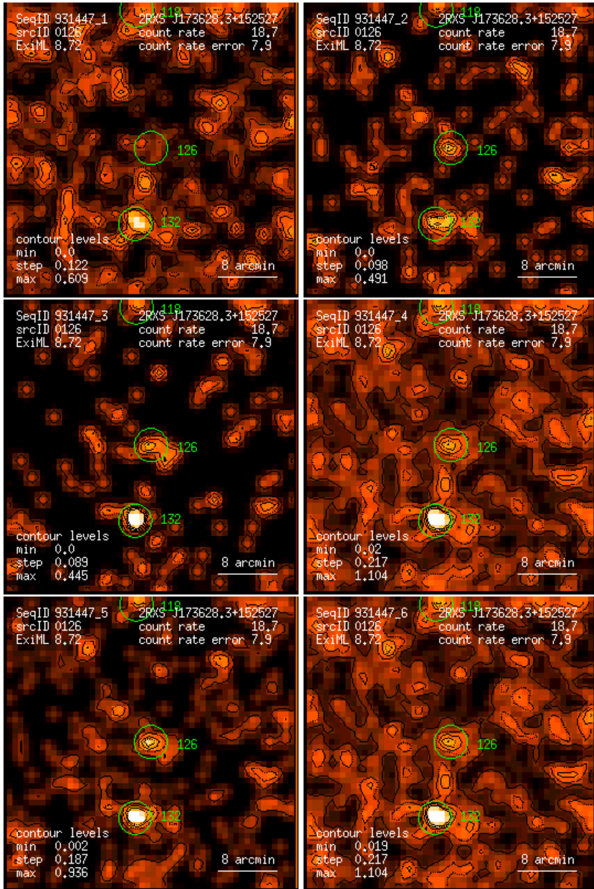
Figure 126: RASS 931447: detection 0126: band rate images, Gaussian filter: (1) PSPC channels 11 – 41, (2) 52 – 90, (3) 91 – 201, (4) 11 – 235, (5) 52 – 201, (6) 11 – 201. Broad band rates in counts/ks. Band rate contour levels in counts/ks/arcmin 2 .
