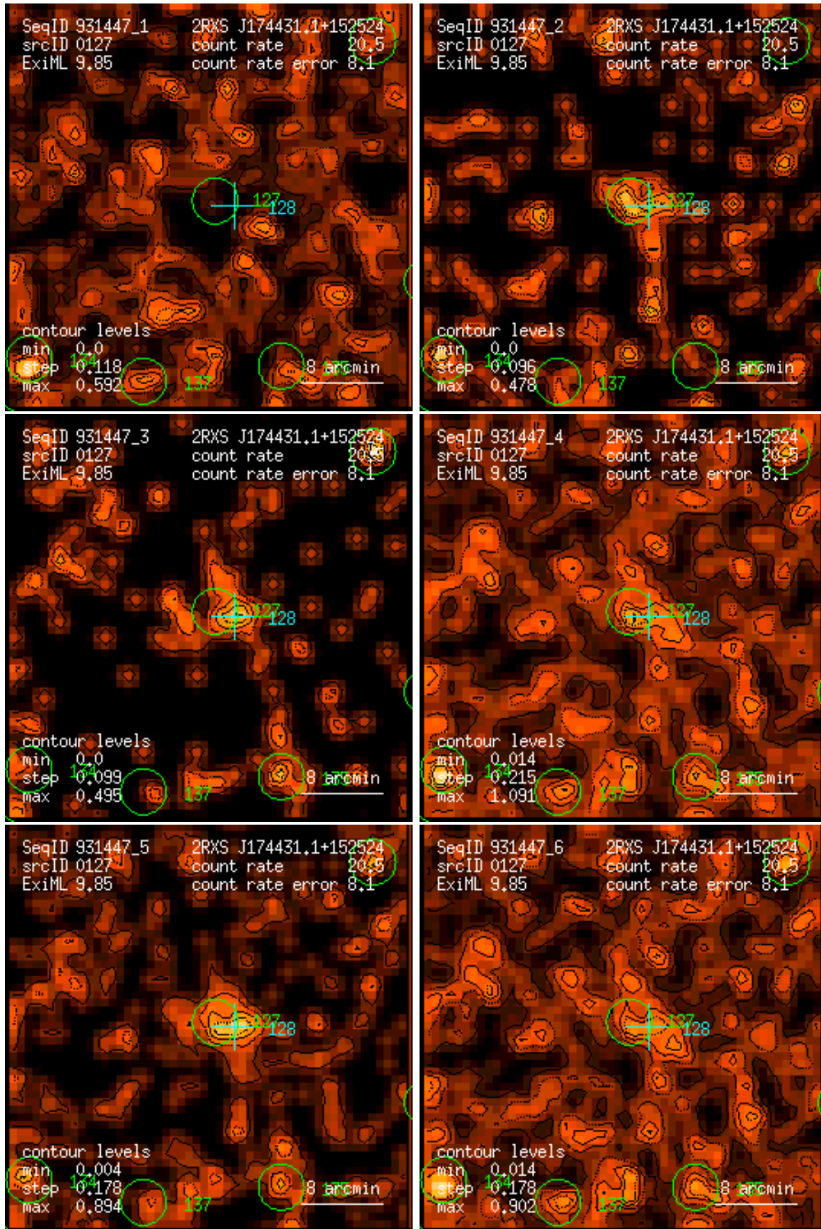
Figure 127: RASS 931447: detection 0127: band rate images, Gaussian filter: (1) PSPC channels 11 – 41, (2) 52 – 90, (3) 91 – 201, (4) 11 – 235, (5) 52 – 201, (6) 11 – 201. Broad band rates in counts/ks. Band rate contour levels in counts/ks/arcmin 2 .
