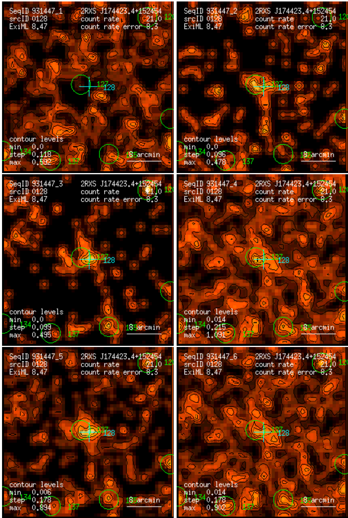
Figure 128: RASS 931447: detection 0128: band rate images, Gaussian filter: (1) PSPC channels 11 – 41, (2) 52 – 90, (3) 91 – 201, (4) 11 – 235, (5) 52 – 201, (6) 11 – 201. Broad band rates in counts/ks. Band rate contour levels in counts/ks/arcmin 2 .
