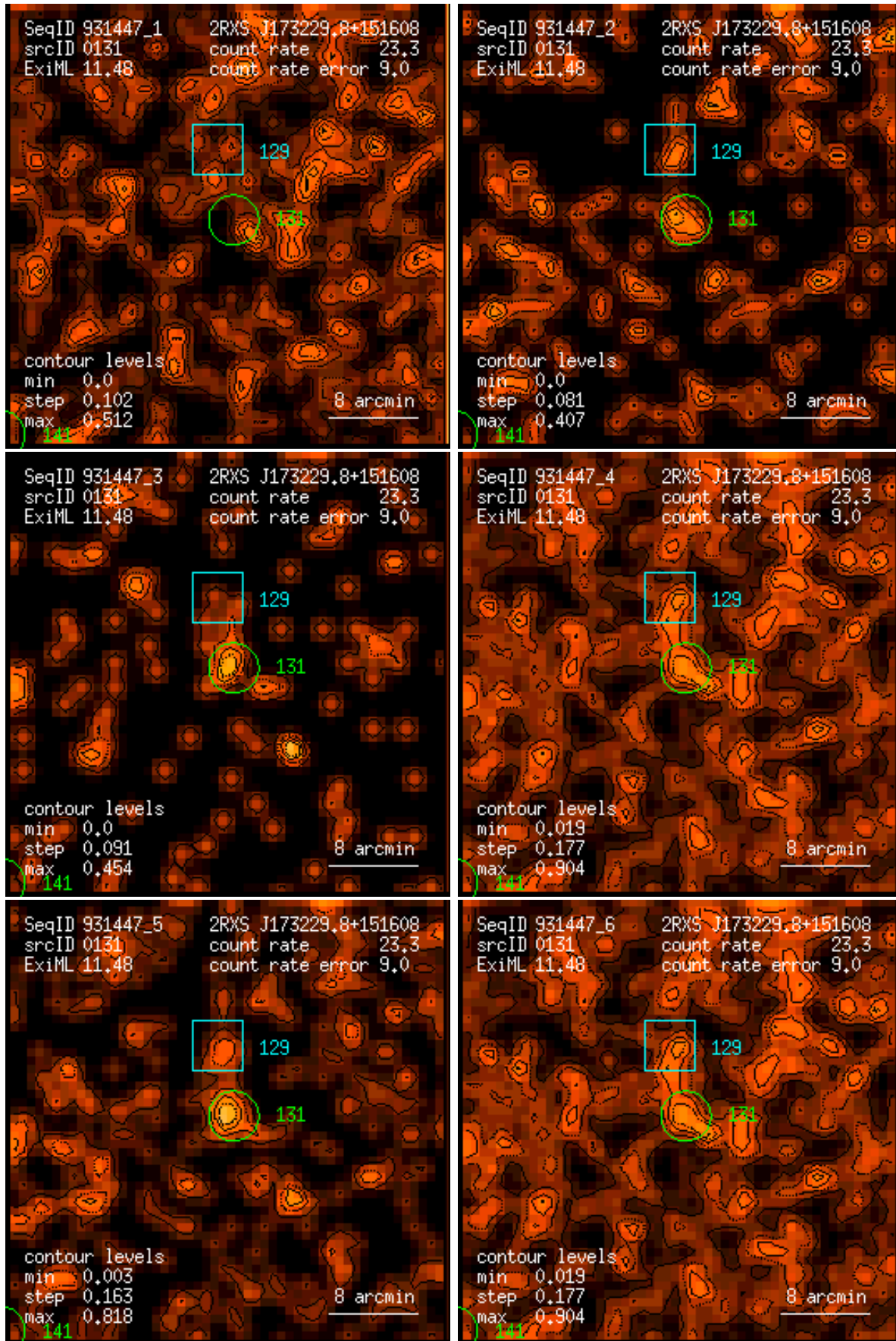
Figure 131: RASS 931447: detection 0131: band rate images, Gaussian filter: (1) PSPC channels 11 – 41, (2) 52 – 90, (3) 91 – 201, (4) 11 – 235, (5) 52 – 201, (6) 11 – 201. Broad band rates in counts/ks. Band rate contour levels in counts/ks/arcmin 2 .
