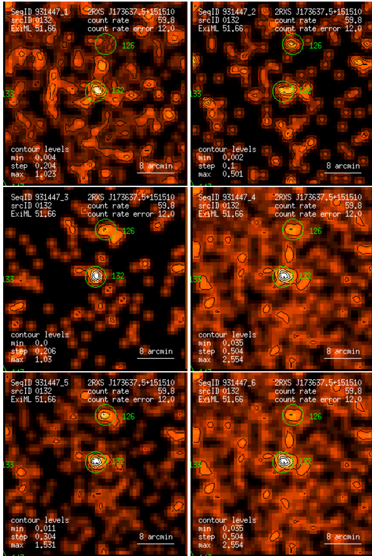
Figure 132: RASS 931447: detection 0132: band rate images, Gaussian filter: (1) PSPC channels 11 – 41, (2) 52 – 90, (3) 91 – 201, (4) 11 – 235, (5) 52 – 201, (6) 11 – 201. Broad band rates in counts/ks. Band rate contour levels in counts/ks/arcmin 2 .
