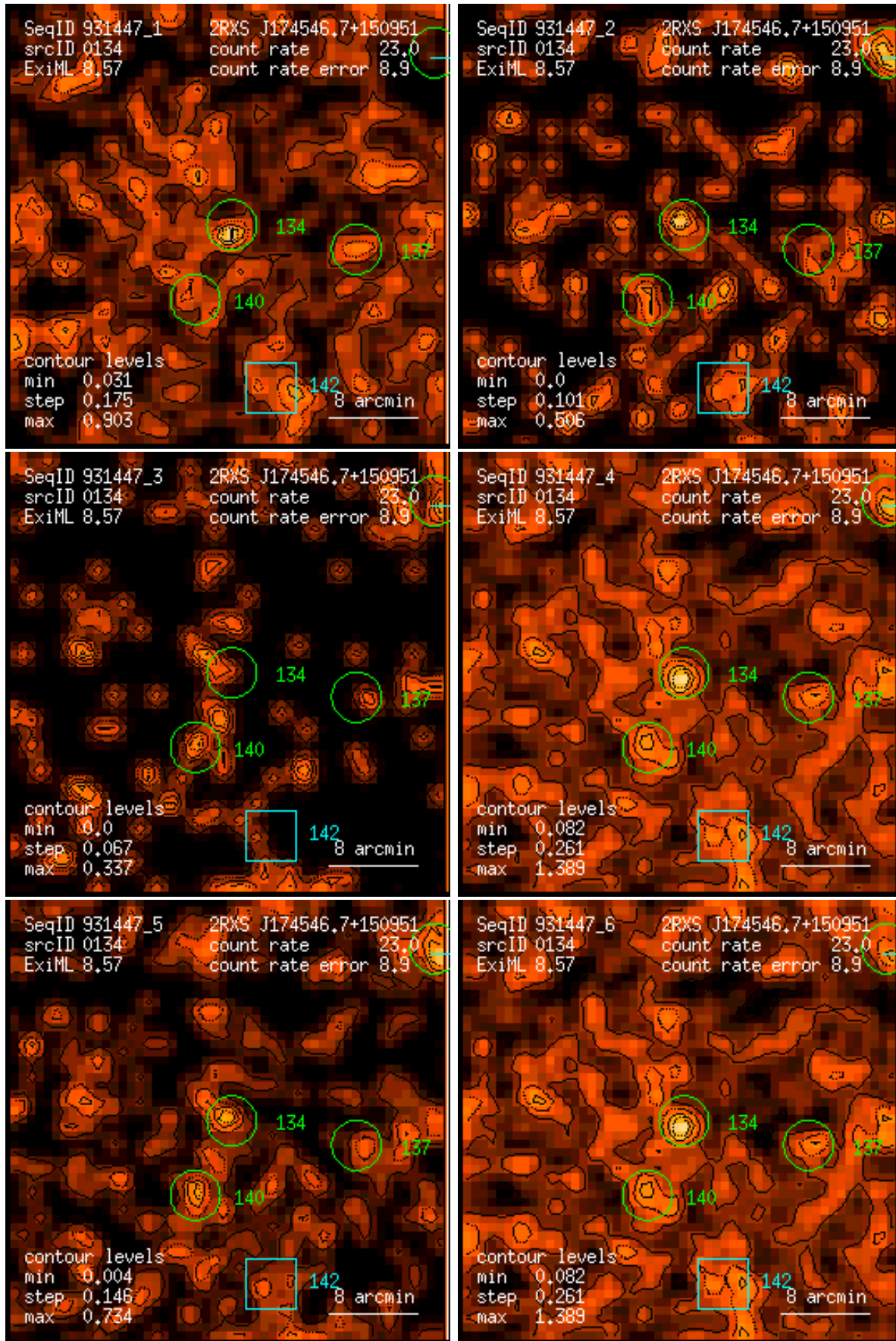
Figure 134: RASS 931447: detection 0134: band rate images, Gaussian filter: (1) PSPC channels 11 – 41, (2) 52 – 90, (3) 91 – 201, (4) 11 – 235, (5) 52 – 201, (6) 11 – 201. Broad band rates in counts/ks. Band rate contour levels in counts/ks/arcmin 2 .
