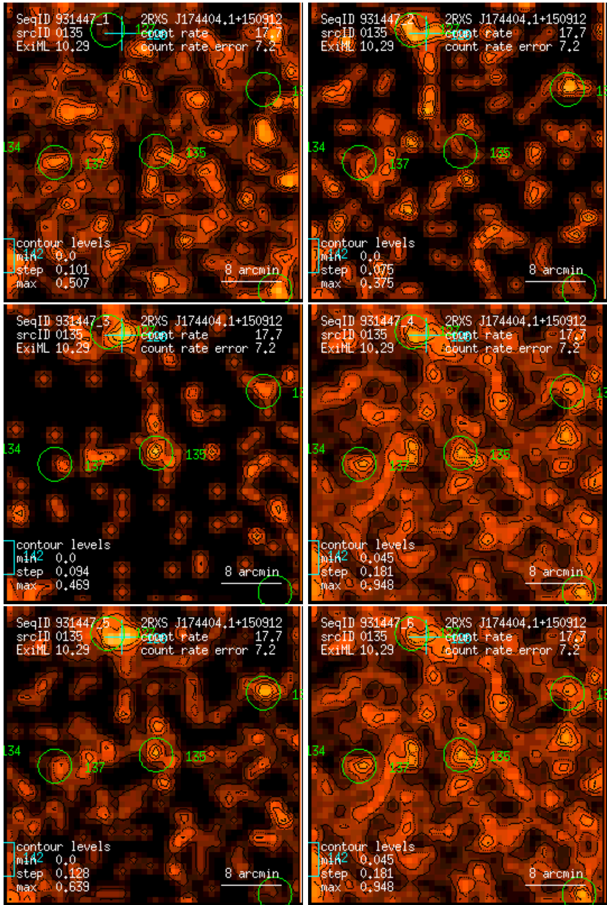
Figure 135: RASS 931447: detection 0135: band rate images, Gaussian filter: (1) PSPC channels 11 – 41, (2) 52 – 90, (3) 91 – 201, (4) 11 – 235, (5) 52 – 201, (6) 11 – 201. Broad band rates in counts/ks. Band rate contour levels in counts/ks/arcmin 2 .
