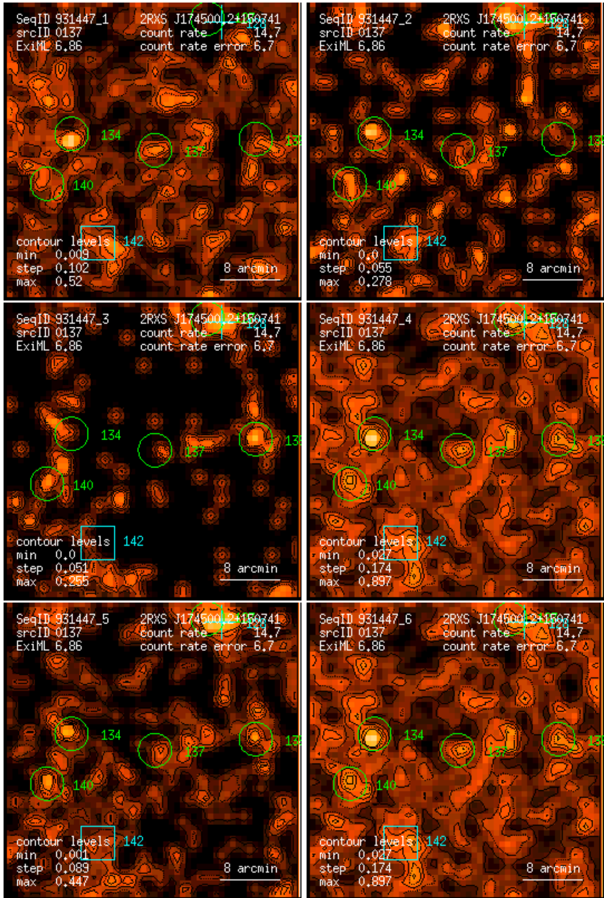
Figure 137: RASS 931447: detection 0137: band rate images, Gaussian filter: (1) PSPC channels 11 – 41, (2) 52 – 90, (3) 91 – 201, (4) 11 – 235, (5) 52 – 201, (6) 11 – 201. Broad band rates in counts/ks. Band rate contour levels in counts/ks/arcmin 2 .
