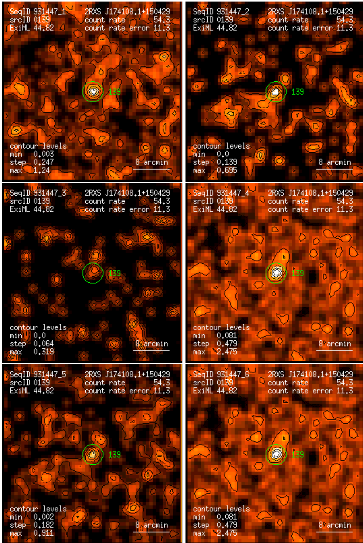
Figure 139: RASS 931447: detection 0139: band rate images, Gaussian filter: (1) PSPC channels 11 – 41, (2) 52 – 90, (3) 91 – 201, (4) 11 – 235, (5) 52 – 201, (6) 11 – 201. Broad band rates in counts/ks. Band rate contour levels in counts/ks/arcmin 2 .
