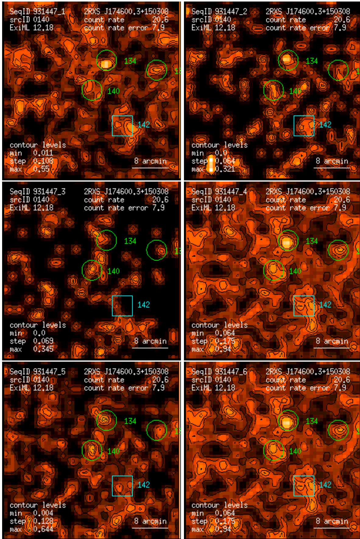
Figure 140: RASS 931447: detection 0140: band rate images, Gaussian filter: (1) PSPC channels 11 – 41, (2) 52 – 90, (3) 91 – 201, (4) 11 – 235, (5) 52 – 201, (6) 11 – 201. Broad band rates in counts/ks. Band rate contour levels in counts/ks/arcmin 2 .
