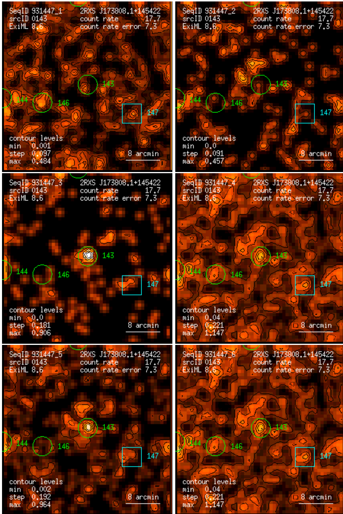
Figure 143: RASS 931447: detection 0143: band rate images, Gaussian filter: (1) PSPC channels 11 – 41, (2) 52 – 90, (3) 91 – 201, (4) 11 – 235, (5) 52 – 201, (6) 11 – 201. Broad band rates in counts/ks. Band rate contour levels in counts/ks/arcmin 2 .
