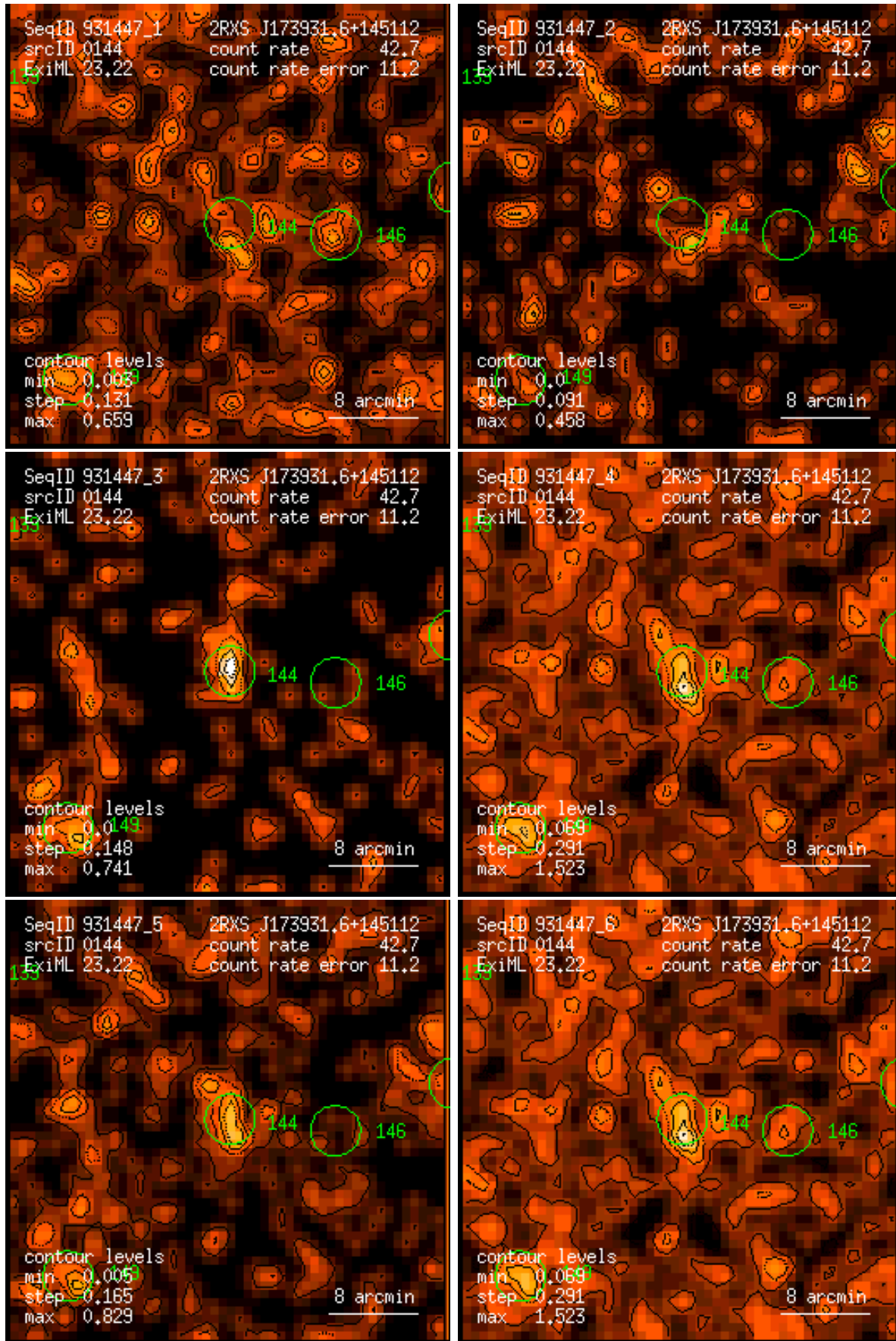
Figure 144: RASS 931447: detection 0144: band rate images, Gaussian filter: (1) PSPC channels 11 – 41, (2) 52 – 90, (3) 91 – 201, (4) 11 – 235, (5) 52 – 201, (6) 11 – 201. Broad band rates in counts/ks. Band rate contour levels in counts/ks/arcmin 2 .
