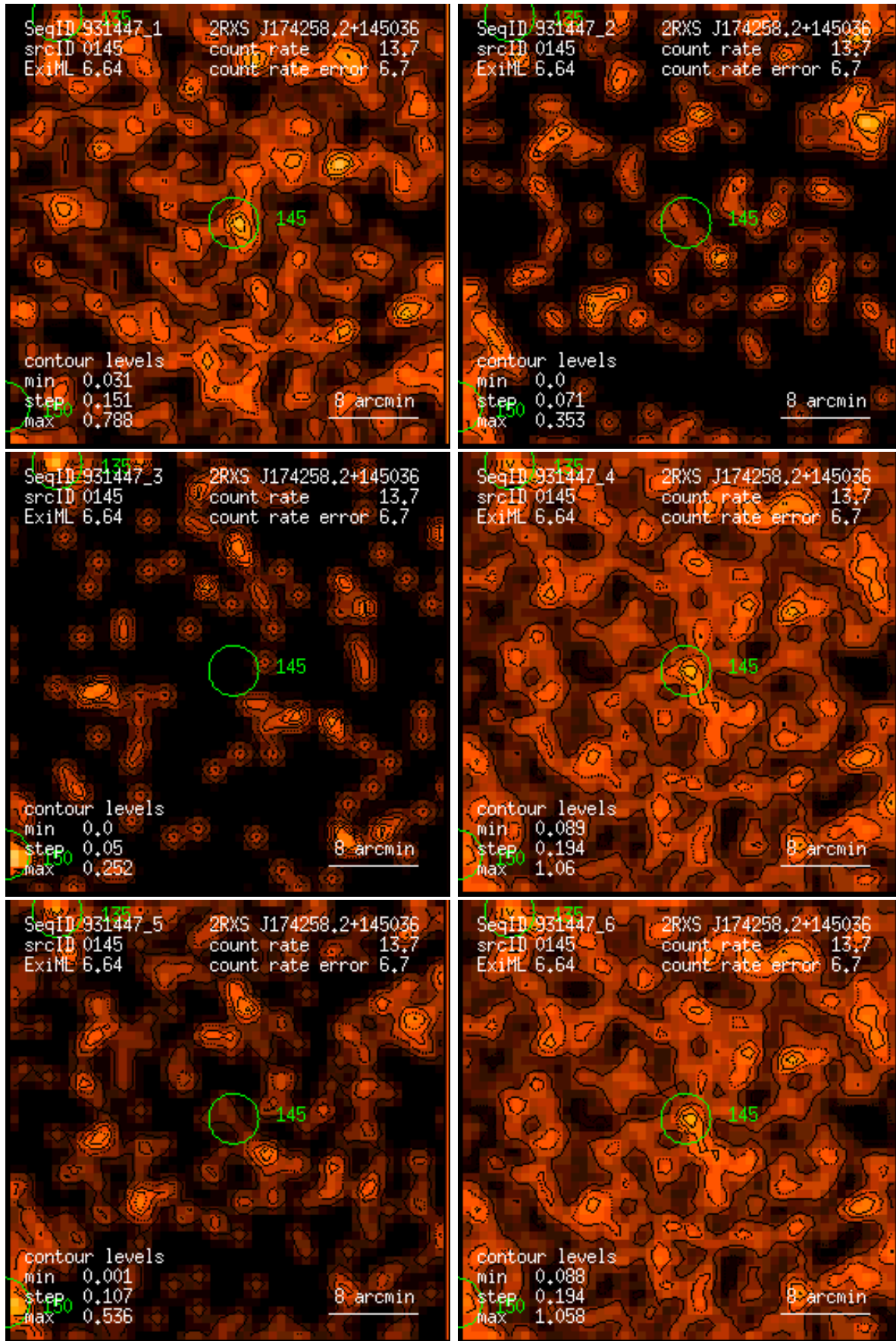
Figure 145: RASS 931447: detection 0145: band rate images, Gaussian filter: (1) PSPC channels 11 – 41, (2) 52 – 90, (3) 91 – 201, (4) 11 – 235, (5) 52 – 201, (6) 11 – 201. Broad band rates in counts/ks. Band rate contour levels in counts/ks/arcmin 2 .
