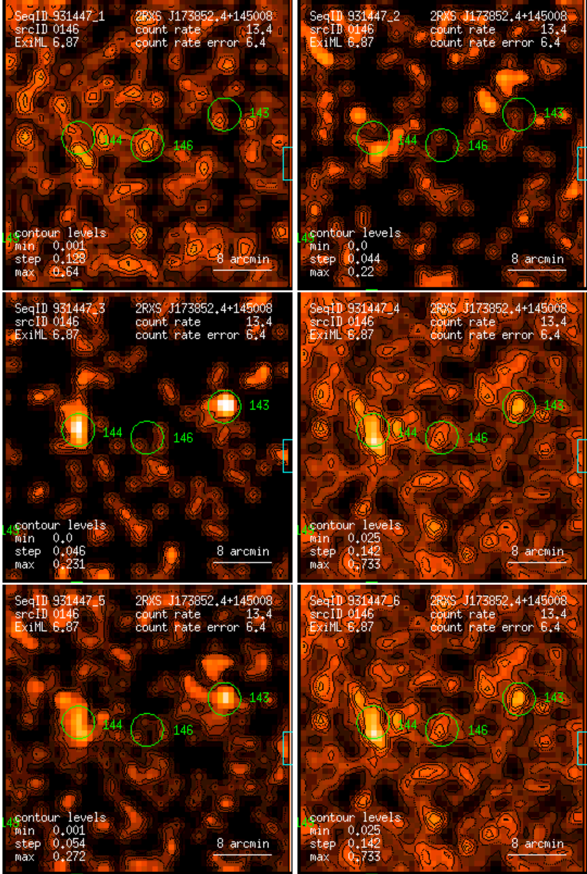
Figure 146: RASS 931447: detection 0146: band rate images, Gaussian filter: (1) PSPC channels 11 – 41, (2) 52 – 90, (3) 91 – 201, (4) 11 – 235, (5) 52 – 201, (6) 11 – 201. Broad band rates in counts/ks. Band rate contour levels in counts/ks/arcmin 2 .
