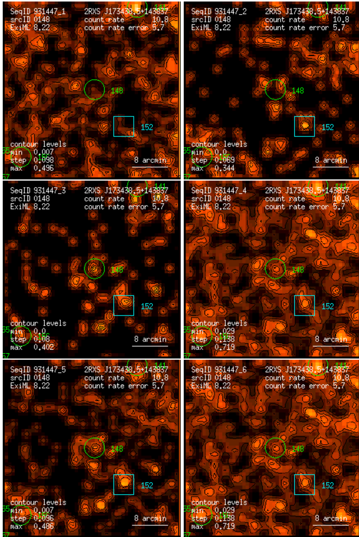
Figure 148: RASS 931447: detection 0148: band rate images, Gaussian filter: (1) PSPC channels 11 – 41, (2) 52 – 90, (3) 91 – 201, (4) 11 – 235, (5) 52 – 201, (6) 11 – 201. Broad band rates in counts/ks. Band rate contour levels in counts/ks/arcmin 2 .
