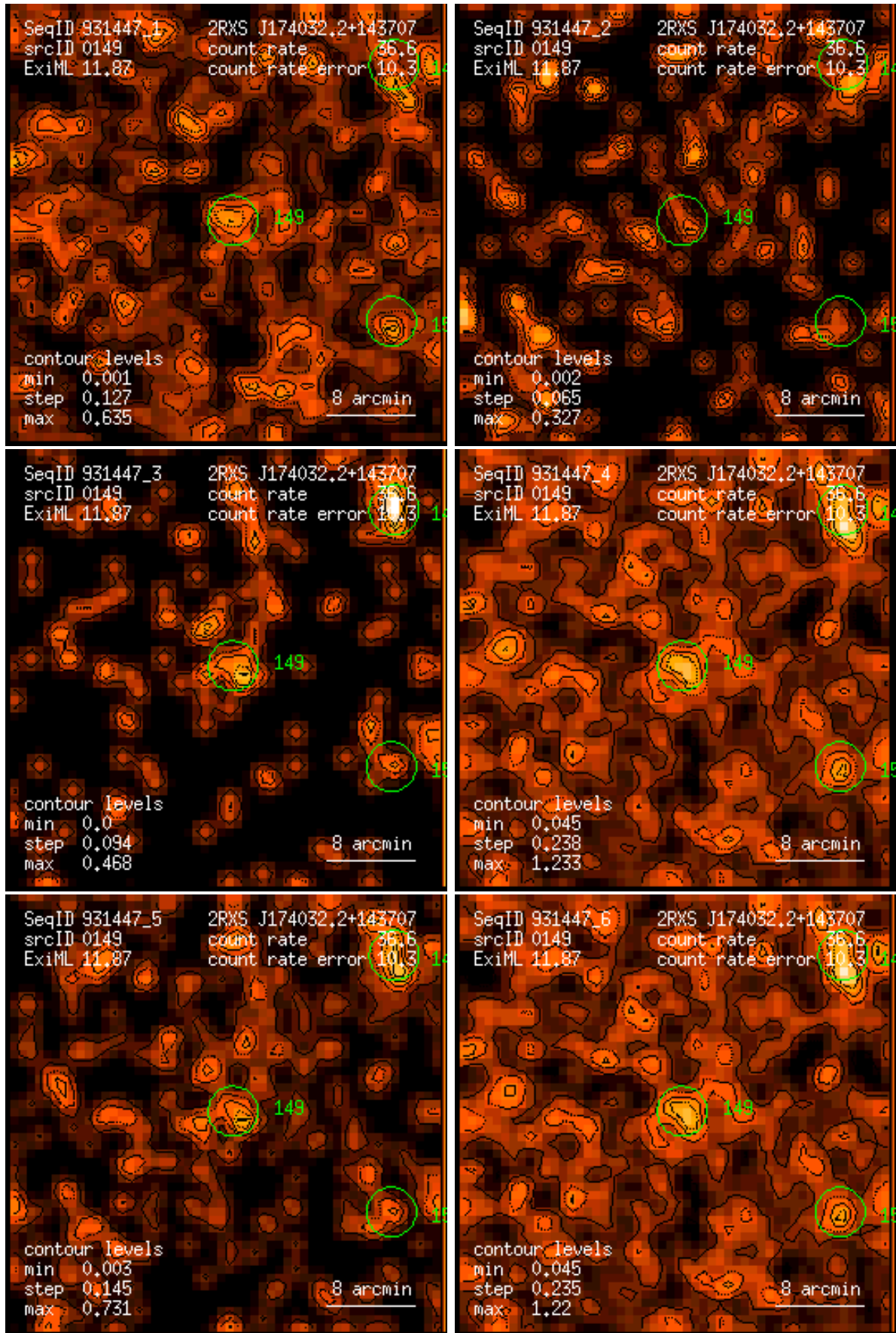
Figure 149: RASS 931447: detection 0149: band rate images, Gaussian filter: (1) PSPC channels 11 – 41, (2) 52 – 90, (3) 91 – 201, (4) 11 – 235, (5) 52 – 201, (6) 11 – 201. Broad band rates in counts/ks. Band rate contour levels in counts/ks/arcmin 2 .
