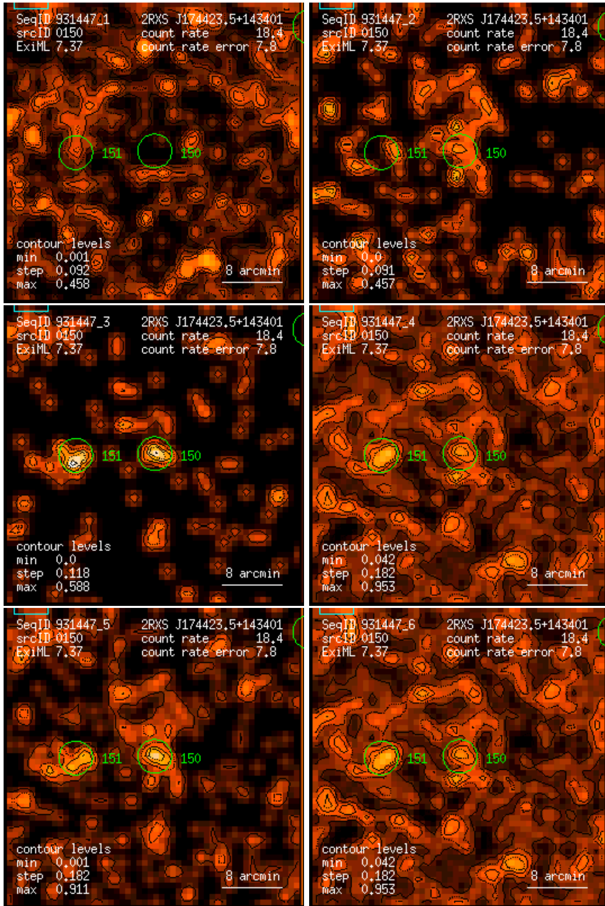
Figure 150: RASS 931447: detection 0150: band rate images, Gaussian filter: (1) PSPC channels 11 – 41, (2) 52 – 90, (3) 91 – 201, (4) 11 – 235, (5) 52 – 201, (6) 11 – 201. Broad band rates in counts/ks. Band rate contour levels in counts/ks/arcmin 2 .
