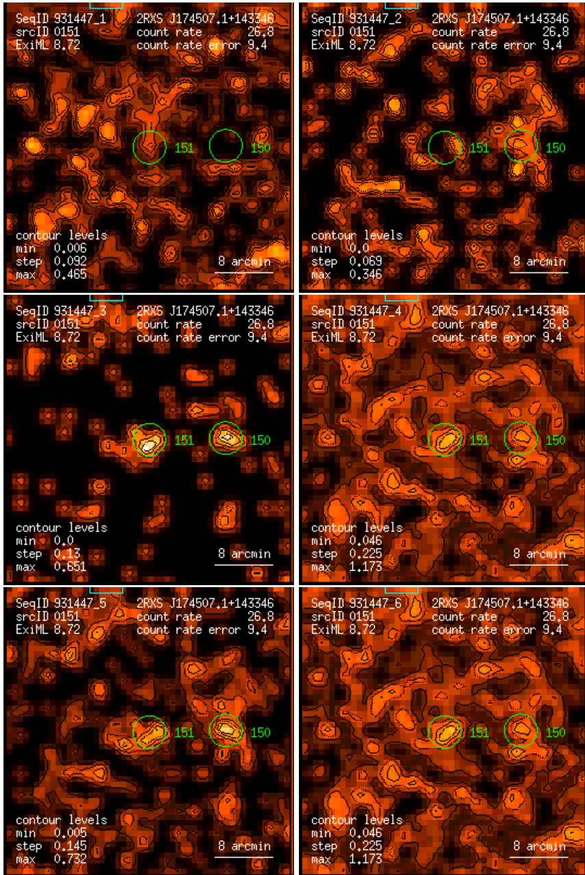
Figure 151: RASS 931447: detection 0151: band rate images, Gaussian filter: (1) PSPC channels 11 – 41, (2) 52 – 90, (3) 91 – 201, (4) 11 – 235, (5) 52 – 201, (6) 11 – 201. Broad band rates in counts/ks. Band rate contour levels in counts/ks/arcmin 2 .
