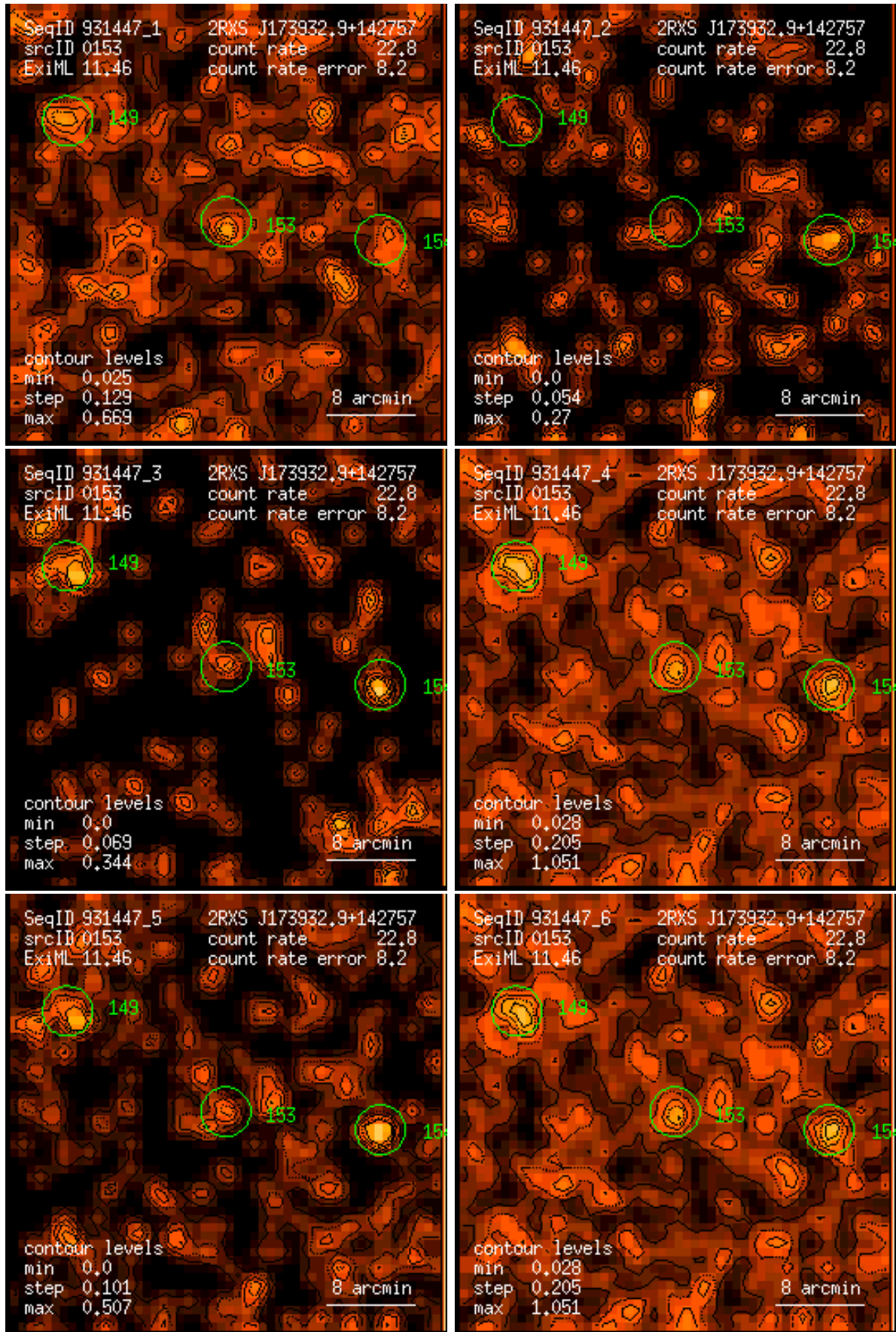
Figure 153: RASS 931447: detection 0153: band rate images, Gaussian filter: (1) PSPC channels 11 – 41, (2) 52 – 90, (3) 91 – 201, (4) 11 – 235, (5) 52 – 201, (6) 11 – 201. Broad band rates in counts/ks. Band rate contour levels in counts/ks/arcmin 2 .
