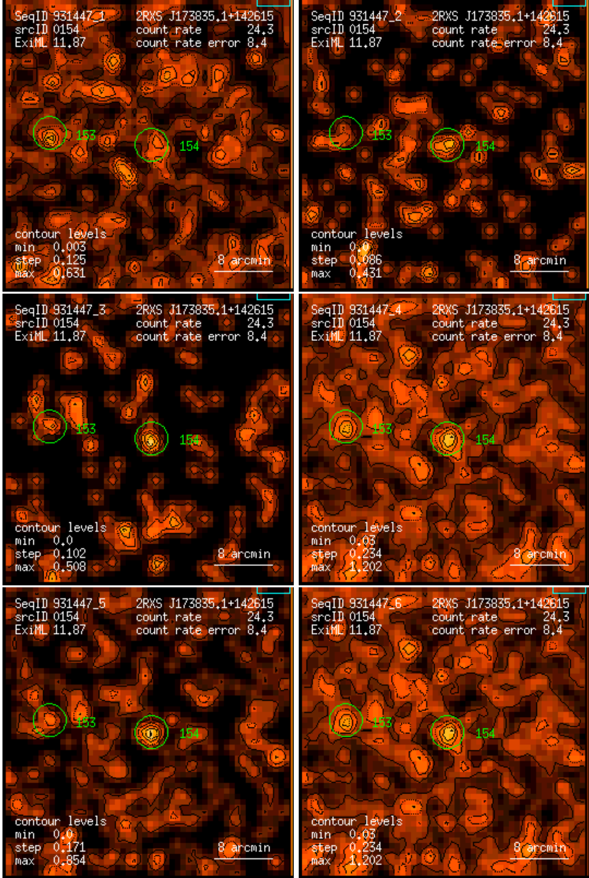
Figure 154: RASS 931447: detection 0154: band rate images, Gaussian filter: (1) PSPC channels 11 – 41, (2) 52 – 90, (3) 91 – 201, (4) 11 – 235, (5) 52 – 201, (6) 11 – 201. Broad band rates in counts/ks. Band rate contour levels in counts/ks/arcmin 2 .
