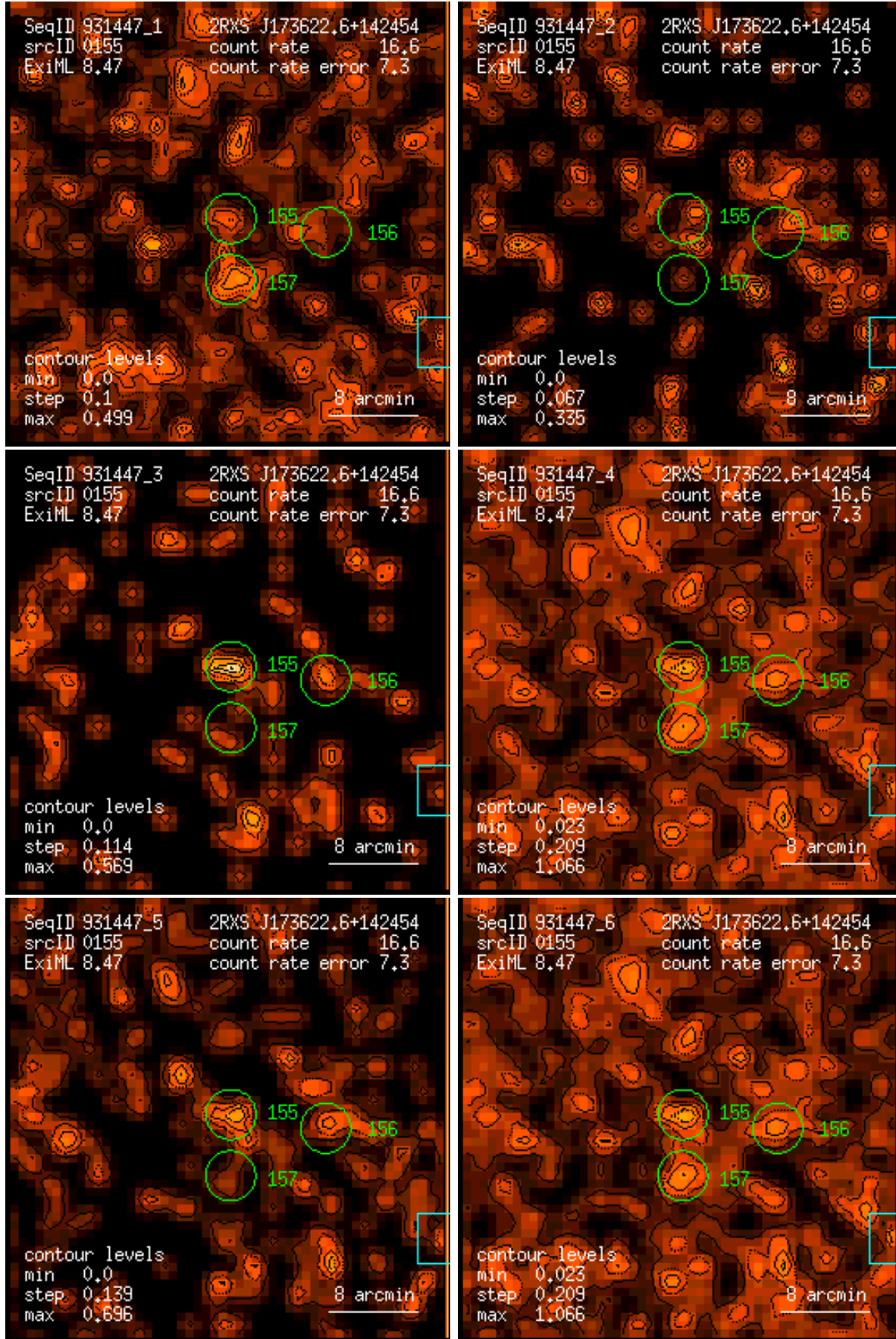
Figure 155: RASS 931447: detection 0155: band rate images, Gaussian filter: (1) PSPC channels 11 – 41, (2) 52 – 90, (3) 91 – 201, (4) 11 – 235, (5) 52 – 201, (6) 11 – 201. Broad band rates in counts/ks. Band rate contour levels in counts/ks/arcmin 2 .
