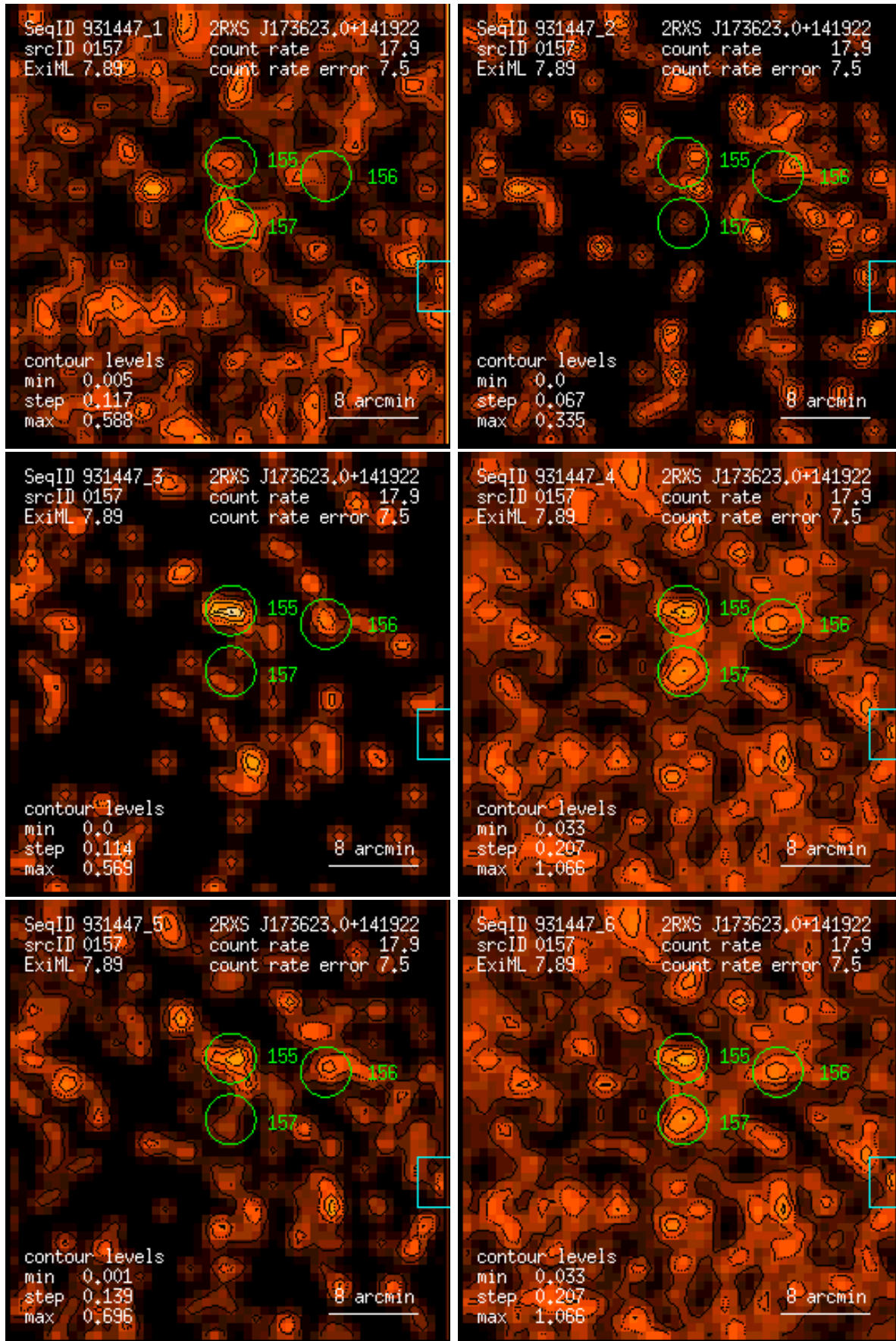
Figure 157: RASS 931447: detection 0157: band rate images, Gaussian filter: (1) PSPC channels 11 – 41, (2) 52 – 90, (3) 91 – 201, (4) 11 – 235, (5) 52 – 201, (6) 11 – 201. Broad band rates in counts/ks. Band rate contour levels in counts/ks/arcmin 2 .
