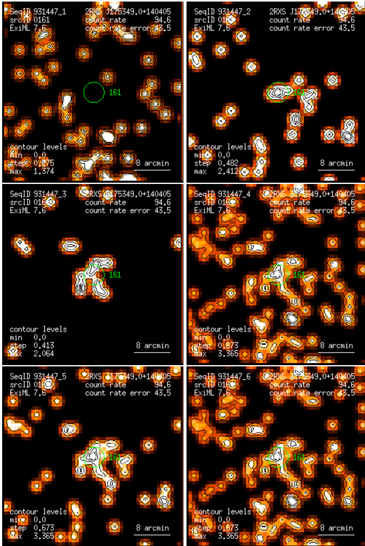
Figure 161: RASS 931447: detection 0161: band rate images, Gaussian filter: (1) PSPC channels 11 – 41, (2) 52 – 90, (3) 91 – 201, (4) 11 – 235, (5) 52 – 201, (6) 11 – 201. Broad band rates in counts/ks. Band rate contour levels in counts/ks/arcmin 2 .
