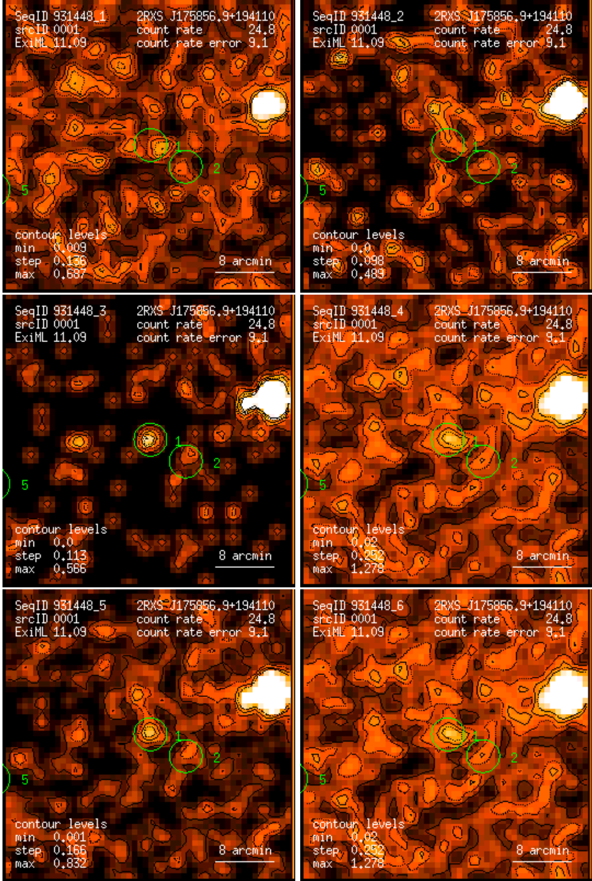
Figure 1: RASS 931448: detection 0001: band rate images, Gaussian filter: (1) PSPC channels 11 – 41, (2) 52 – 90, (3) 91 – 201, (4) 11 – 235, (5) 52 – 201, (6) 11 – 201. Broad band rates in counts/ks. Band rate contour levels in counts/ks/arcmin 2 .
