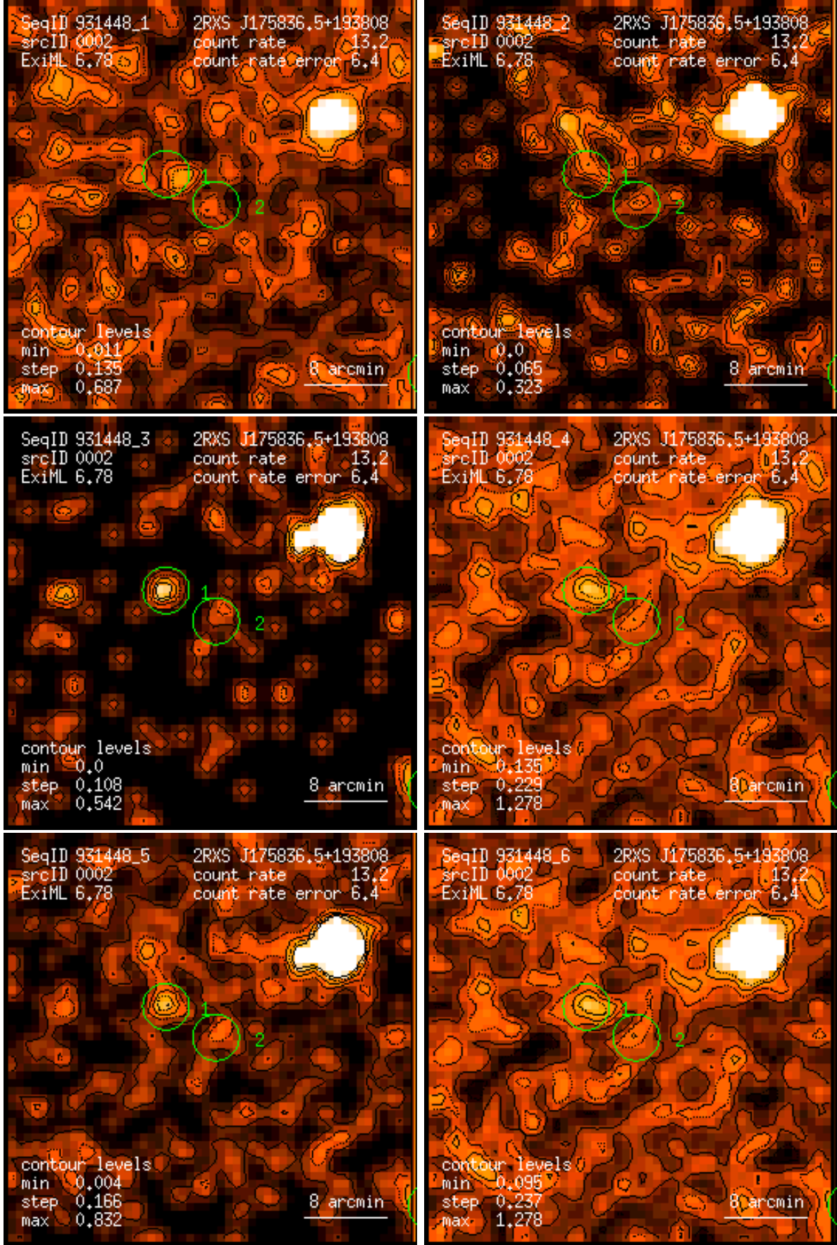
Figure 2: RASS 931448: detection 0002: band rate images, Gaussian filter: (1) PSPC channels 11 – 41, (2) 52 – 90, (3) 91 – 201, (4) 11 – 235, (5) 52 – 201, (6) 11 – 201. Broad band rates in counts/ks. Band rate contour levels in counts/ks/arcmin 2 .
